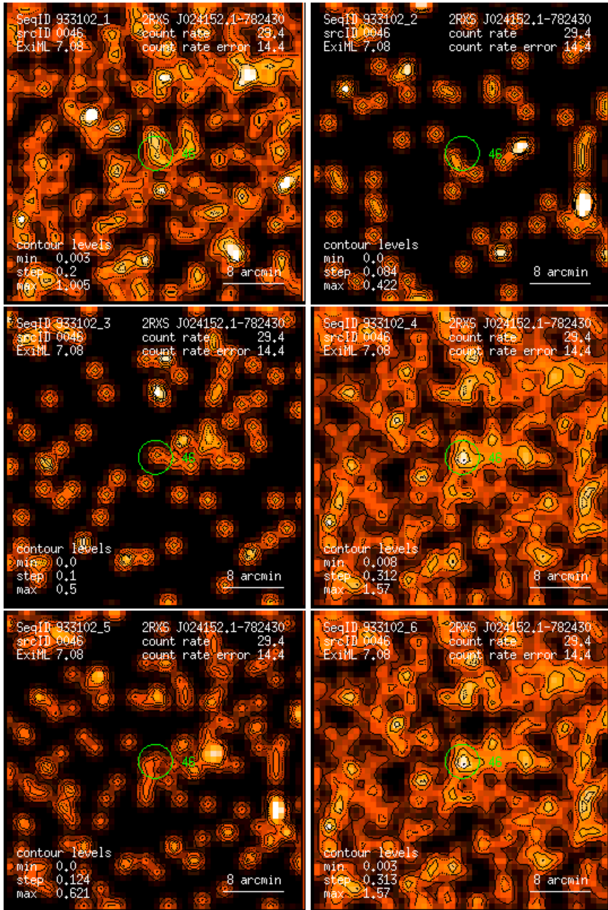
Figure 46: RASS 933102: detection 0046: band rate images, Gaussian filter: (1) PSPC channels 11 – 41, (2) 52 – 90, (3) 91 – 201, (4) 11 – 235, (5) 52 – 201, (6) 11 – 201. Broad band rates in counts/ks. Band rate contour levels in counts/ks/arcmin 2 .
