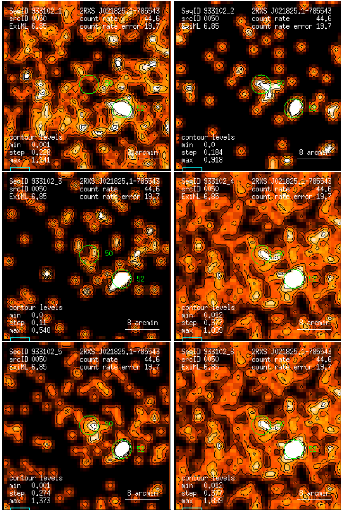
Figure 50: RASS 933102: detection 0050: band rate images, Gaussian filter: (1) PSPC channels 11 – 41, (2) 52 – 90, (3) 91 – 201, (4) 11 – 235, (5) 52 – 201, (6) 11 – 201. Broad band rates in counts/ks. Band rate contour levels in counts/ks/arcmin 2 .
