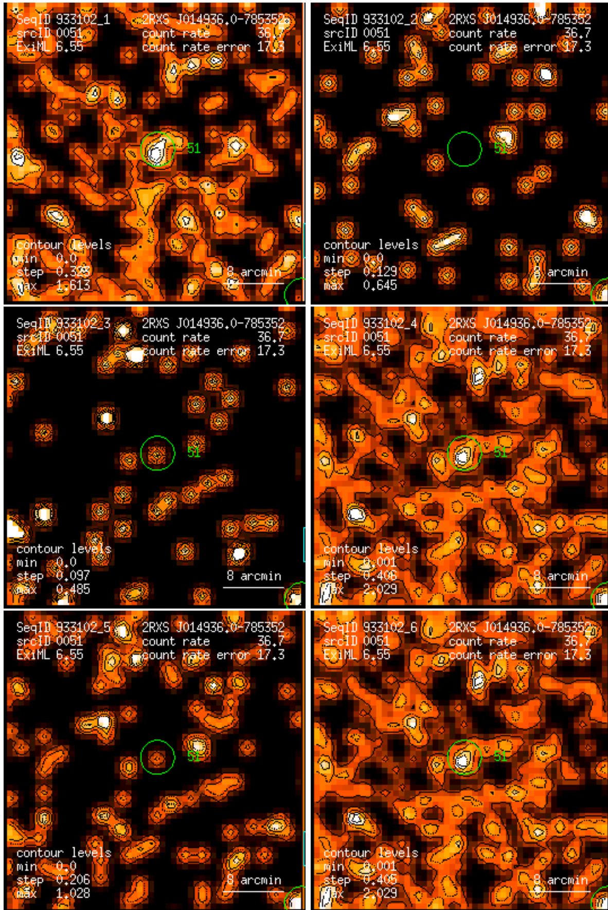
Figure 51: RASS 933102: detection 0051: band rate images, Gaussian filter: (1) PSPC channels 11 – 41, (2) 52 – 90, (3) 91 – 201, (4) 11 – 235, (5) 52 – 201, (6) 11 – 201. Broad band rates in counts/ks. Band rate contour levels in counts/ks/arcmin 2 .
