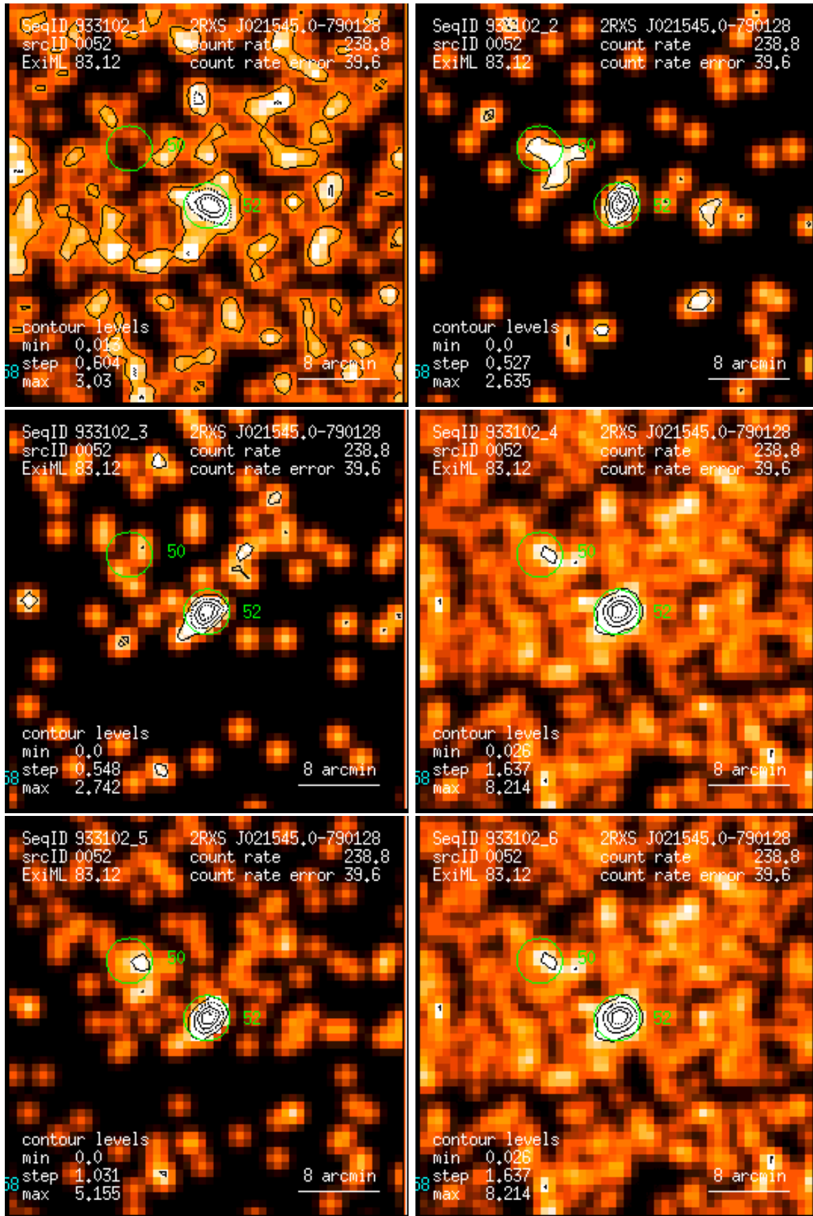
Figure 52: RASS 933102: detection 0052: band rate images, Gaussian filter: (1) PSPC channels 11 – 41, (2) 52 – 90, (3) 91 – 201, (4) 11 – 235, (5) 52 – 201, (6) 11 – 201. Broad band rates in counts/ks. Band rate contour levels in counts/ks/arcmin 2 .
