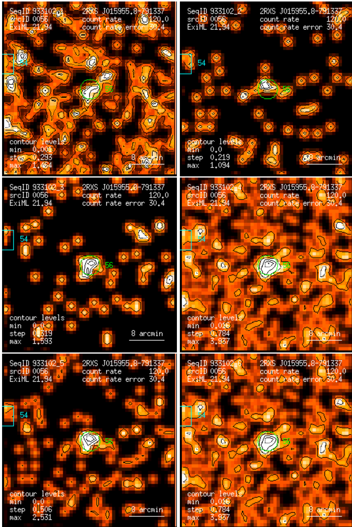
Figure 56: RASS 933102: detection 0056: band rate images, Gaussian filter: (1) PSPC channels 11 – 41, (2) 52 – 90, (3) 91 – 201, (4) 11 – 235, (5) 52 – 201, (6) 11 – 201. Broad band rates in counts/ks. Band rate contour levels in counts/ks/arcmin 2 .
