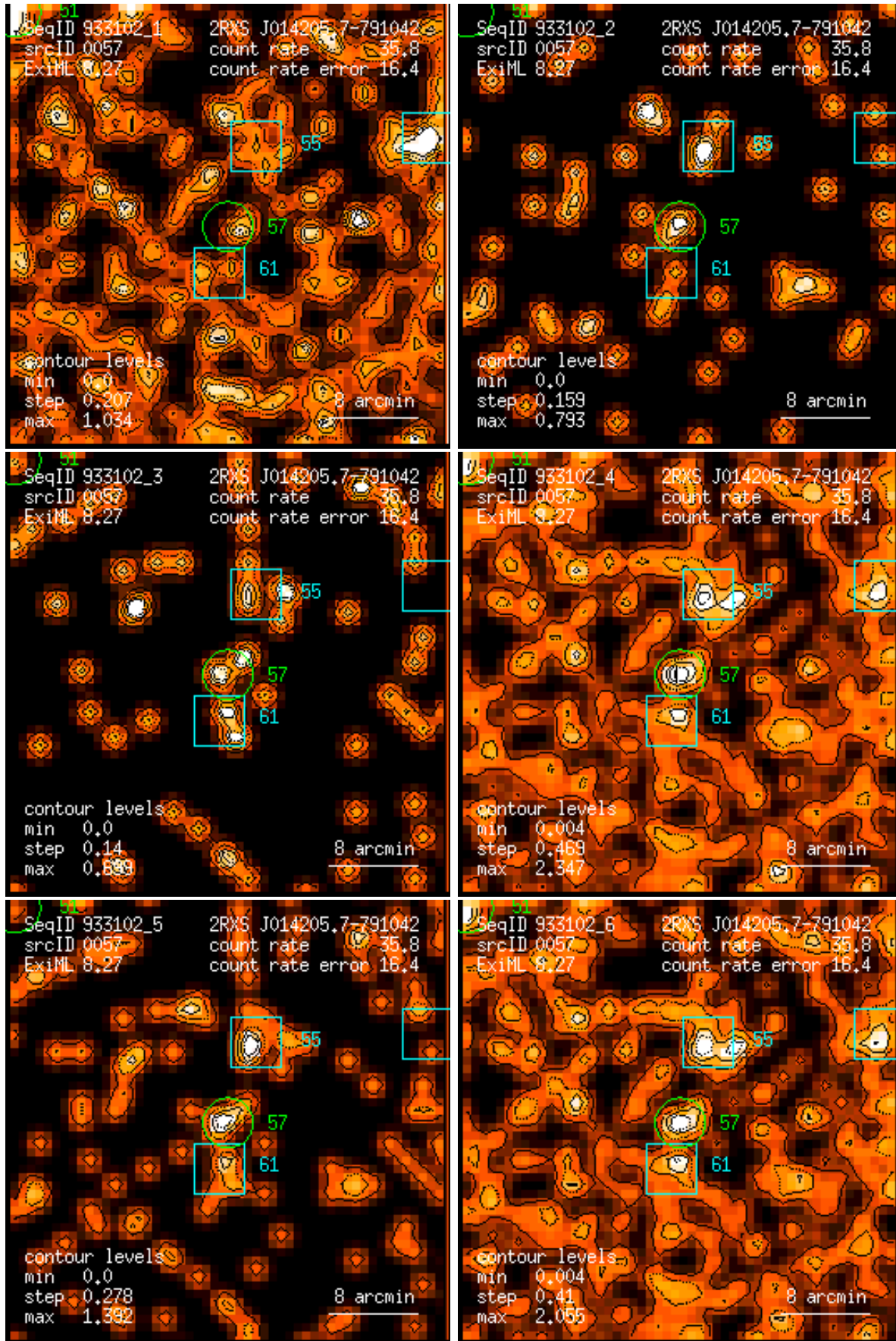
Figure 57: RASS 933102: detection 0057: band rate images, Gaussian filter: (1) PSPC channels 11 – 41, (2) 52 – 90, (3) 91 – 201, (4) 11 – 235, (5) 52 – 201, (6) 11 – 201. Broad band rates in counts/ks. Band rate contour levels in counts/ks/arcmin 2 .
