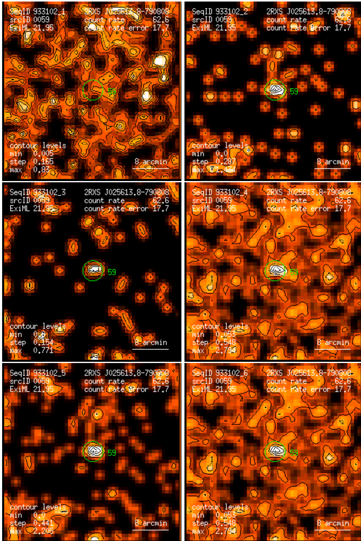
Figure 59: RASS 933102: detection 0059: band rate images, Gaussian filter: (1) PSPC channels 11 – 41, (2) 52 – 90, (3) 91 – 201, (4) 11 – 235, (5) 52 – 201, (6) 11 – 201. Broad band rates in counts/ks. Band rate contour levels in counts/ks/arcmin 2 .
