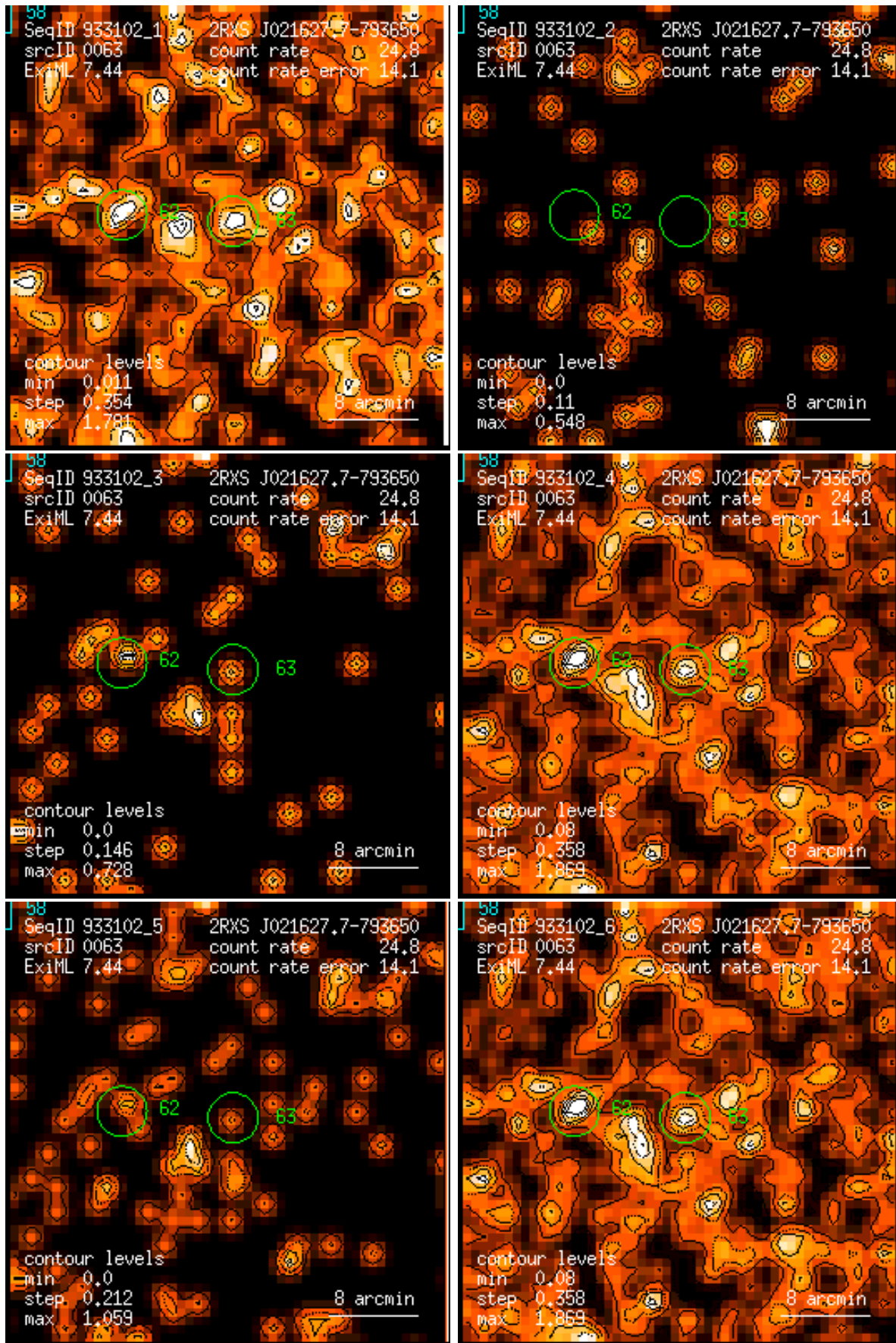
Figure 63: RASS 933102: detection 0063: band rate images, Gaussian filter: (1) PSPC channels 11 – 41, (2) 52 – 90, (3) 91 – 201, (4) 11 – 235, (5) 52 – 201, (6) 11 – 201. Broad band rates in counts/ks. Band rate contour levels in counts/ks/arcmin 2 .
