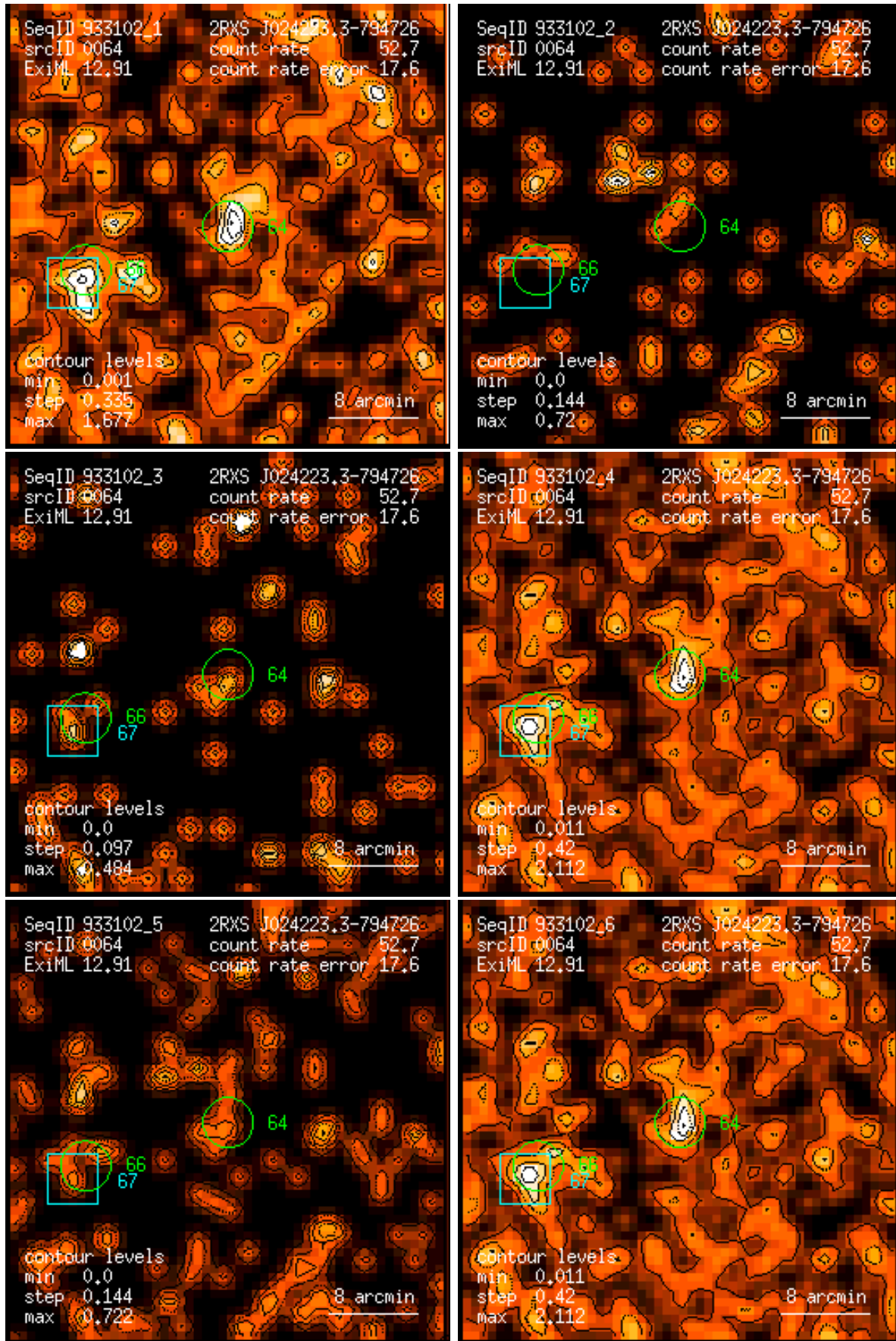
Figure 64: RASS 933102: detection 0064: band rate images, Gaussian filter: (1) PSPC channels 11 – 41, (2) 52 – 90, (3) 91 – 201, (4) 11 – 235, (5) 52 – 201, (6) 11 – 201. Broad band rates in counts/ks. Band rate contour levels in counts/ks/arcmin 2 .
