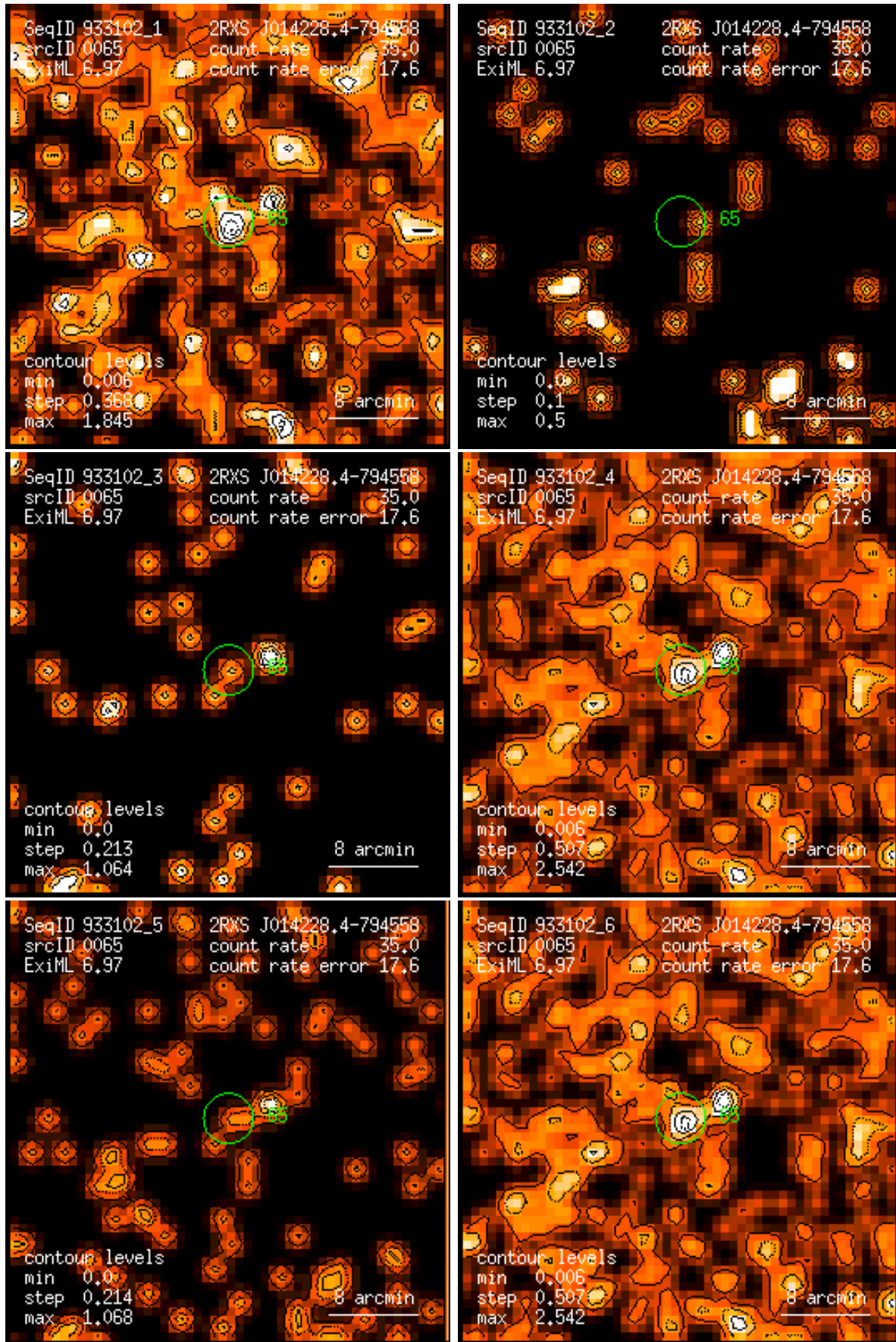
Figure 65: RASS 933102: detection 0065: band rate images, Gaussian filter: (1) PSPC channels 11 – 41, (2) 52 – 90, (3) 91 – 201, (4) 11 – 235, (5) 52 – 201, (6) 11 – 201. Broad band rates in counts/ks. Band rate contour levels in counts/ks/arcmin 2 .
