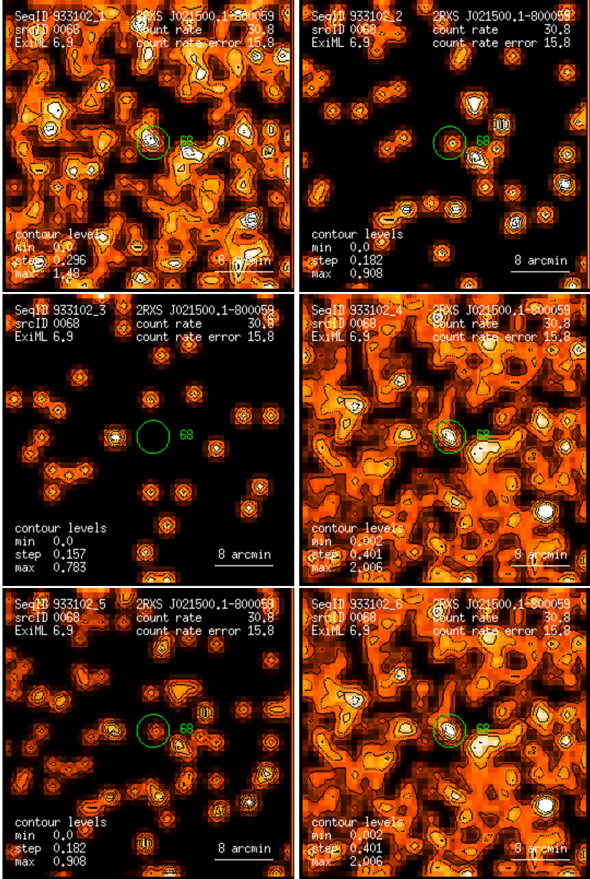
Figure 68: RASS 933102: detection 0068: band rate images, Gaussian filter: (1) PSPC channels 11 – 41, (2) 52 – 90, (3) 91 – 201, (4) 11 – 235, (5) 52 – 201, (6) 11 – 201. Broad band rates in counts/ks. Band rate contour levels in counts/ks/arcmin 2 .
