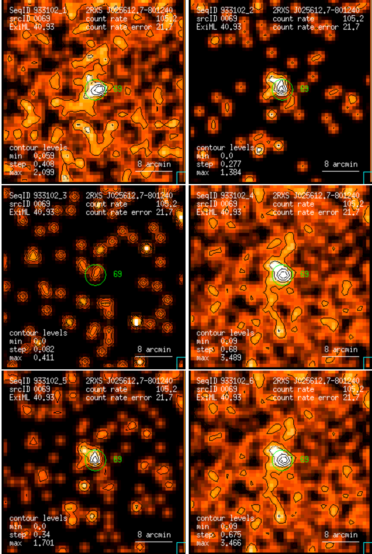
Figure 69: RASS 933102: detection 0069: band rate images, Gaussian filter: (1) PSPC channels 11 – 41, (2) 52 – 90, (3) 91 – 201, (4) 11 – 235, (5) 52 – 201, (6) 11 – 201. Broad band rates in counts/ks. Band rate contour levels in counts/ks/arcmin 2 .
