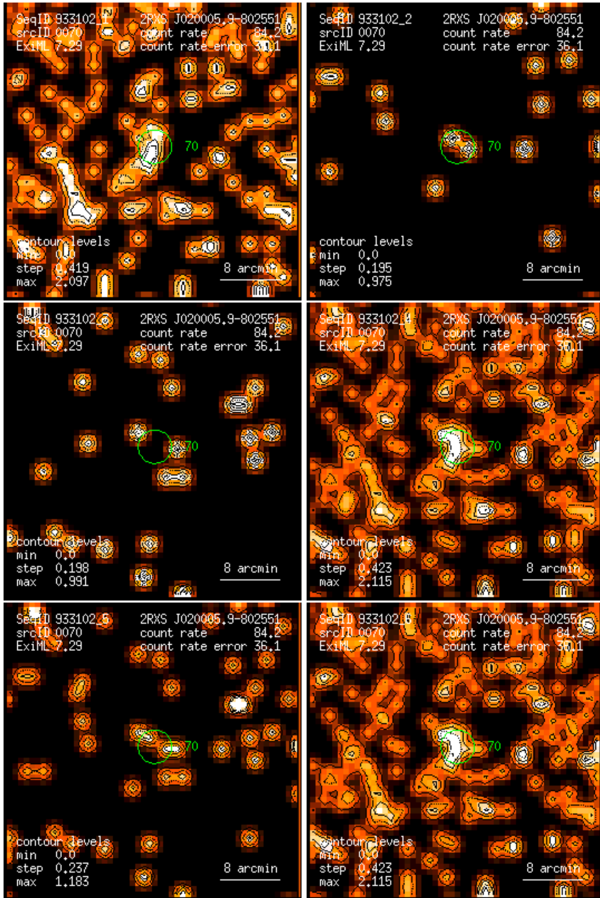
Figure 70: RASS 933102: detection 0070: band rate images, Gaussian filter: (1) PSPC channels 11 – 41, (2) 52 – 90, (3) 91 – 201, (4) 11 – 235, (5) 52 – 201, (6) 11 – 201. Broad band rates in counts/ks. Band rate contour levels in counts/ks/arcmin 2 .
