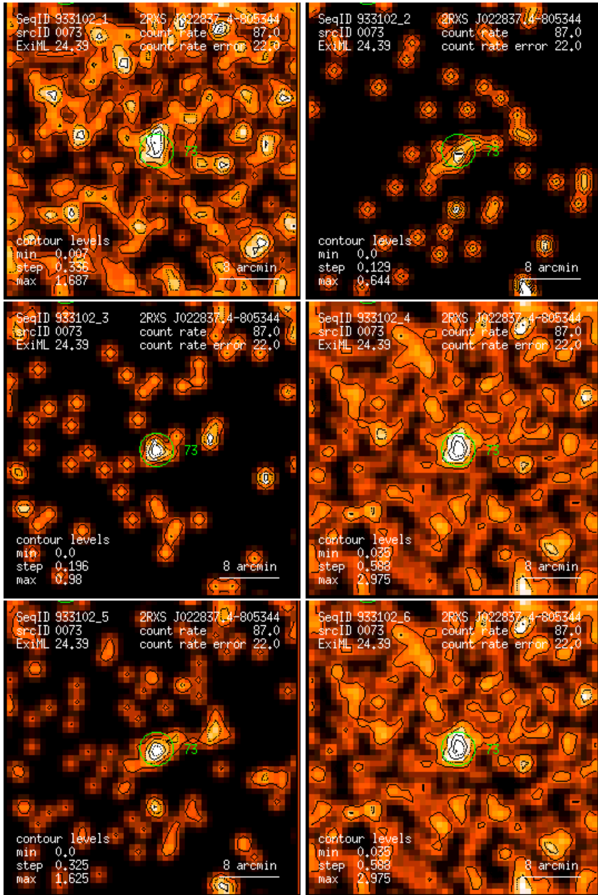
Figure 73: RASS 933102: detection 0073: band rate images, Gaussian filter: (1) PSPC channels 11 – 41, (2) 52 – 90, (3) 91 – 201, (4) 11 – 235, (5) 52 – 201, (6) 11 – 201. Broad band rates in counts/ks. Band rate contour levels in counts/ks/arcmin 2 .
