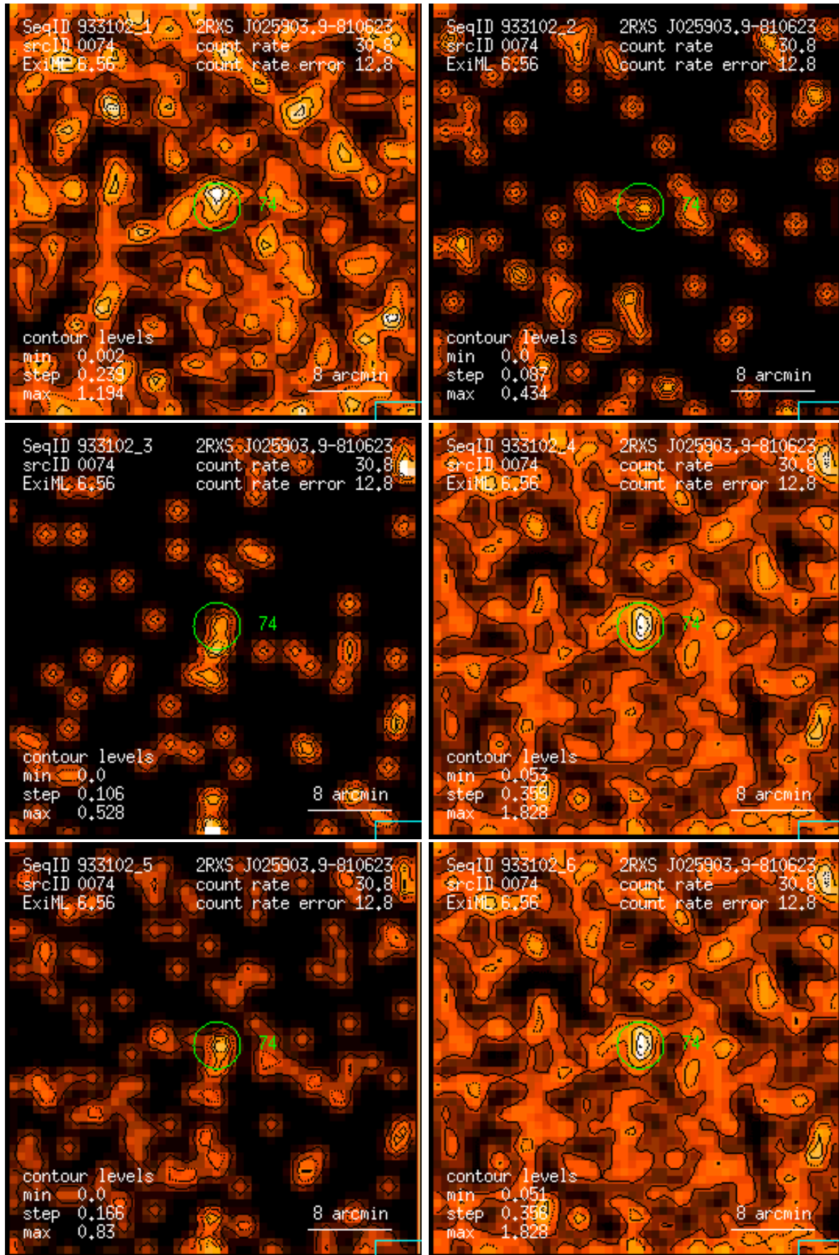
Figure 74: RASS 933102: detection 0074: band rate images, Gaussian filter: (1) PSPC channels 11 – 41, (2) 52 – 90, (3) 91 – 201, (4) 11 – 235, (5) 52 – 201, (6) 11 – 201. Broad band rates in counts/ks. Band rate contour levels in counts/ks/arcmin 2 .
