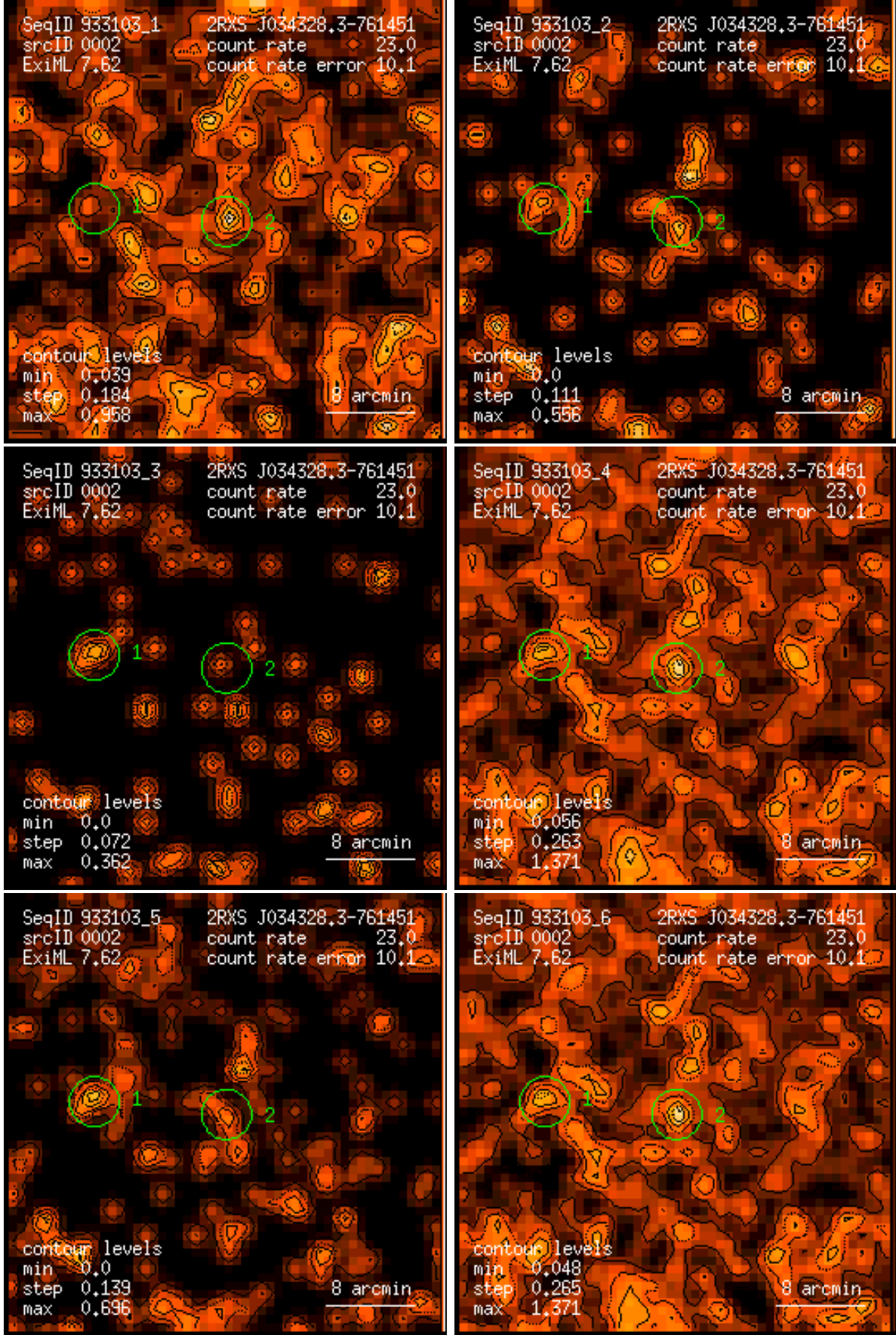
Figure 2: RASS 933103: detection 0002: band rate images, Gaussian filter: (1) PSPC channels 11 – 41, (2) 52 – 90, (3) 91 – 201, (4) 11 – 235, (5) 52 – 201, (6) 11 – 201. Broad band rates in counts/ks. Band rate contour levels in counts/ks/arcmin 2 .
