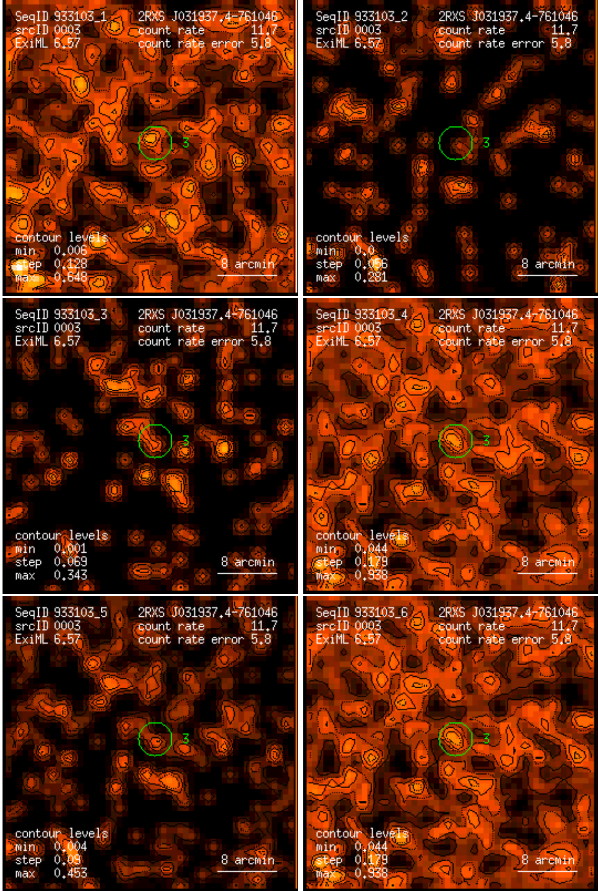
Figure 3: RASS 933103: detection 0003: band rate images, Gaussian filter: (1) PSPC channels 11 – 41, (2) 52 – 90, (3) 91 – 201, (4) 11 – 235, (5) 52 – 201, (6) 11 – 201. Broad band rates in counts/ks. Band rate contour levels in counts/ks/arcmin 2 .
