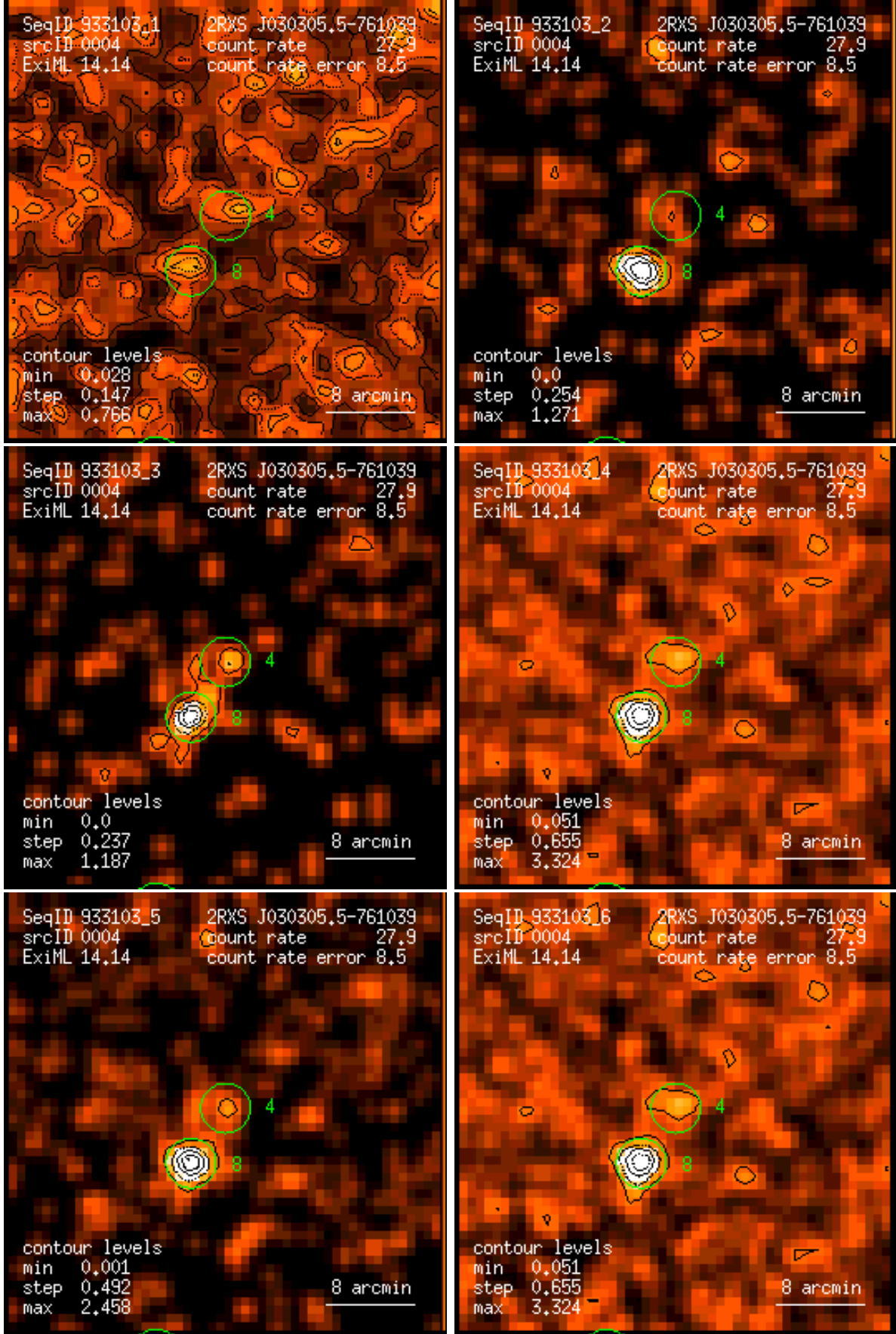
Figure 4: RASS 933103: detection 0004: band rate images, Gaussian filter: (1) PSPC channels 11 – 41, (2) 52 – 90, (3) 91 – 201, (4) 11 – 235, (5) 52 – 201, (6) 11 – 201. Broad band rates in counts/ks. Band rate contour levels in counts/ks/arcmin 2 .
