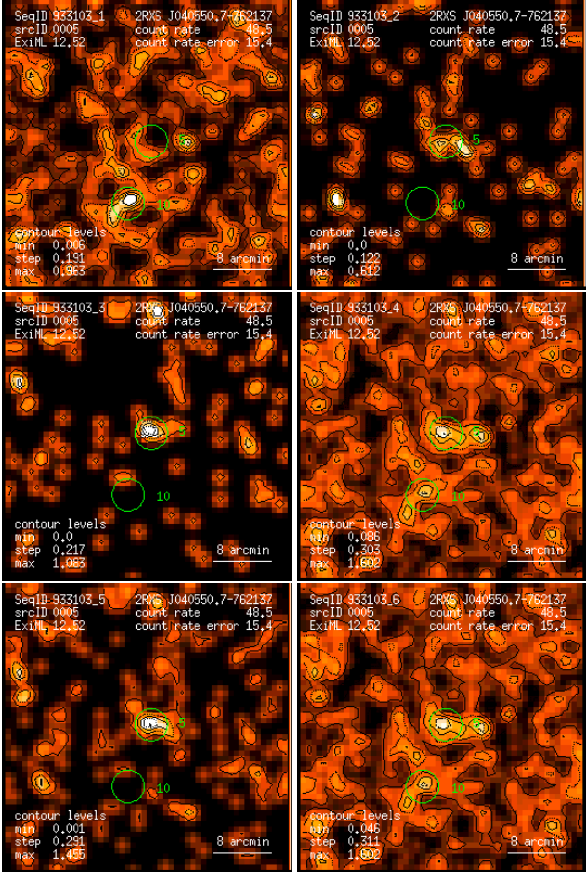
Figure 5: RASS 933103: detection 0005: band rate images, Gaussian filter: (1) PSPC channels 11 – 41, (2) 52 – 90, (3) 91 – 201, (4) 11 – 235, (5) 52 – 201, (6) 11 – 201. Broad band rates in counts/ks. Band rate contour levels in counts/ks/arcmin 2 .
