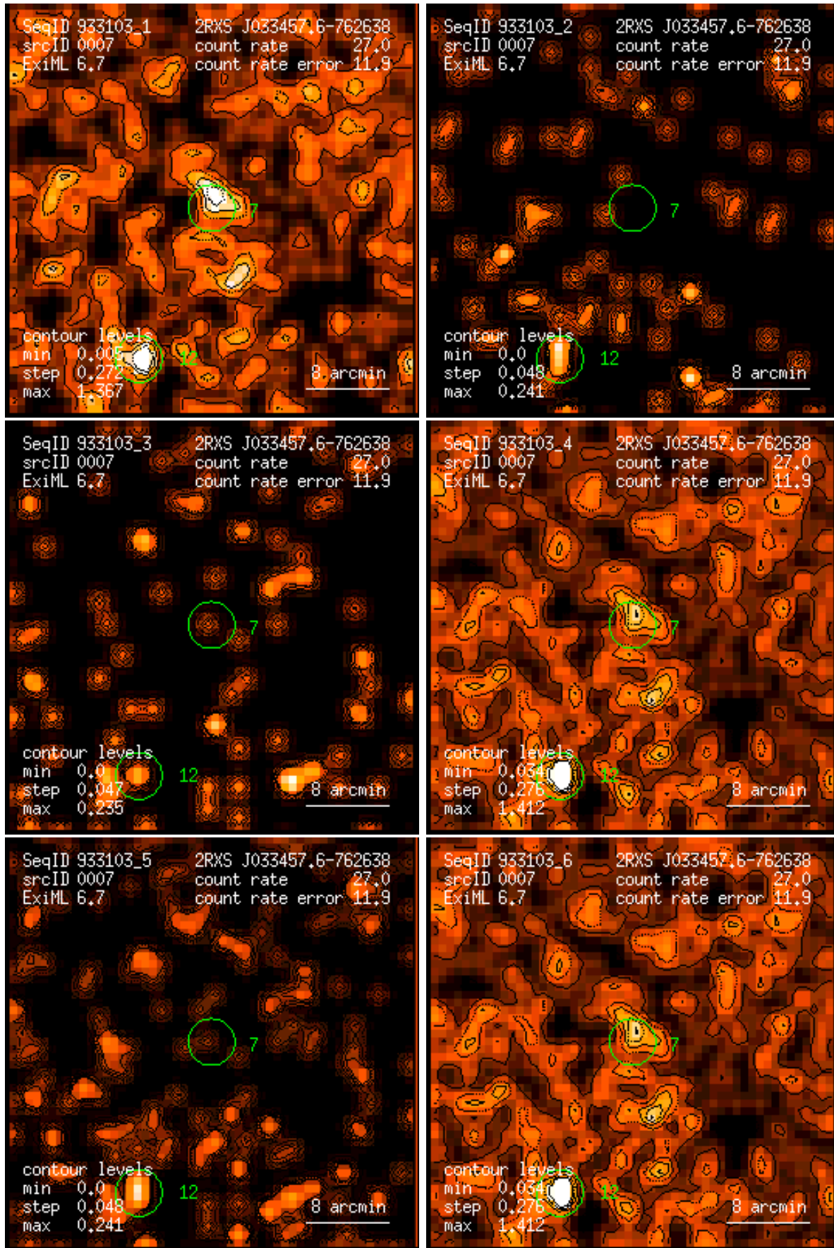
Figure 7: RASS 933103: detection 0007: band rate images, Gaussian filter: (1) PSPC channels 11 – 41, (2) 52 – 90, (3) 91 – 201, (4) 11 – 235, (5) 52 – 201, (6) 11 – 201. Broad band rates in counts/ks. Band rate contour levels in counts/ks/arcmin 2 .
