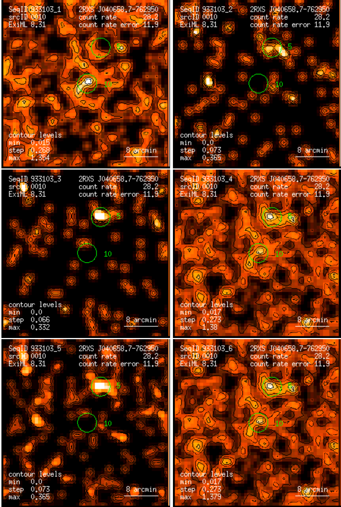
Figure 10: RASS 933103: detection 0010: band rate images, Gaussian filter: (1) PSPC channels 11 – 41, (2) 52 – 90, (3) 91 – 201, (4) 11 – 235, (5) 52 – 201, (6) 11 – 201. Broad band rates in counts/ks. Band rate contour levels in counts/ks/arcmin 2 .
