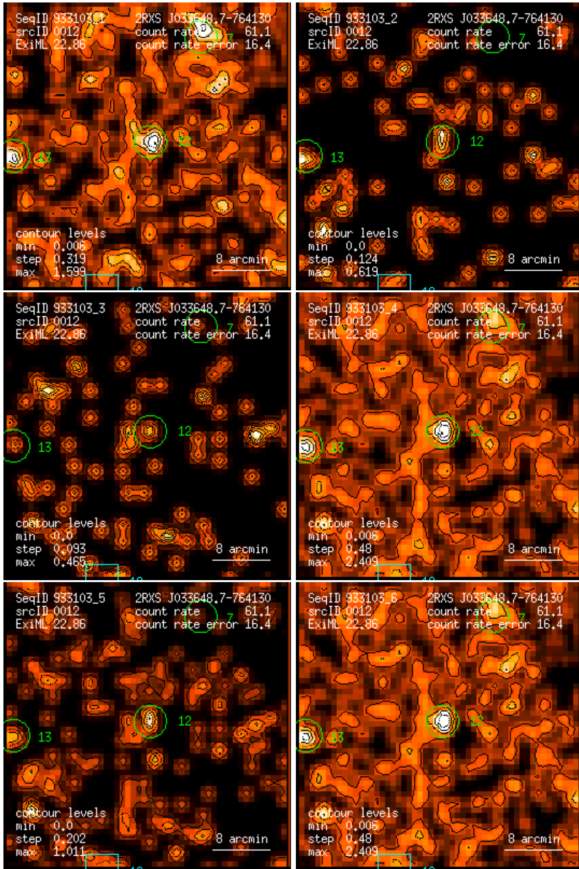
Figure 12: RASS 933103: detection 0012: band rate images, Gaussian filter: (1) PSPC channels 11 – 41, (2) 52 – 90, (3) 91 – 201, (4) 11 – 235, (5) 52 – 201, (6) 11 – 201. Broad band rates in counts/ks. Band rate contour levels in counts/ks/arcmin 2 .
