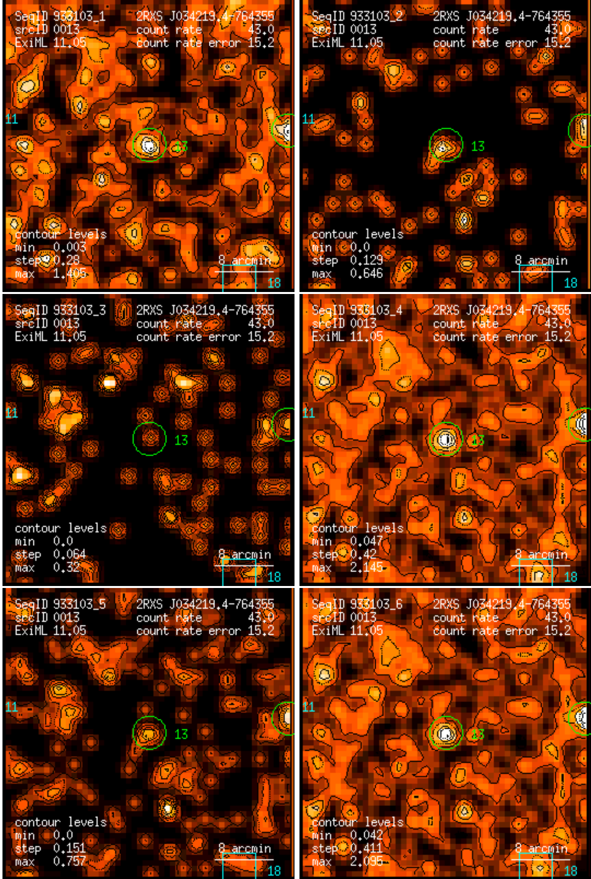
Figure 13: RASS 933103: detection 0013: band rate images, Gaussian filter: (1) PSPC channels 11 – 41, (2) 52 – 90, (3) 91 – 201, (4) 11 – 235, (5) 52 – 201, (6) 11 – 201. Broad band rates in counts/ks. Band rate contour levels in counts/ks/arcmin 2 .
