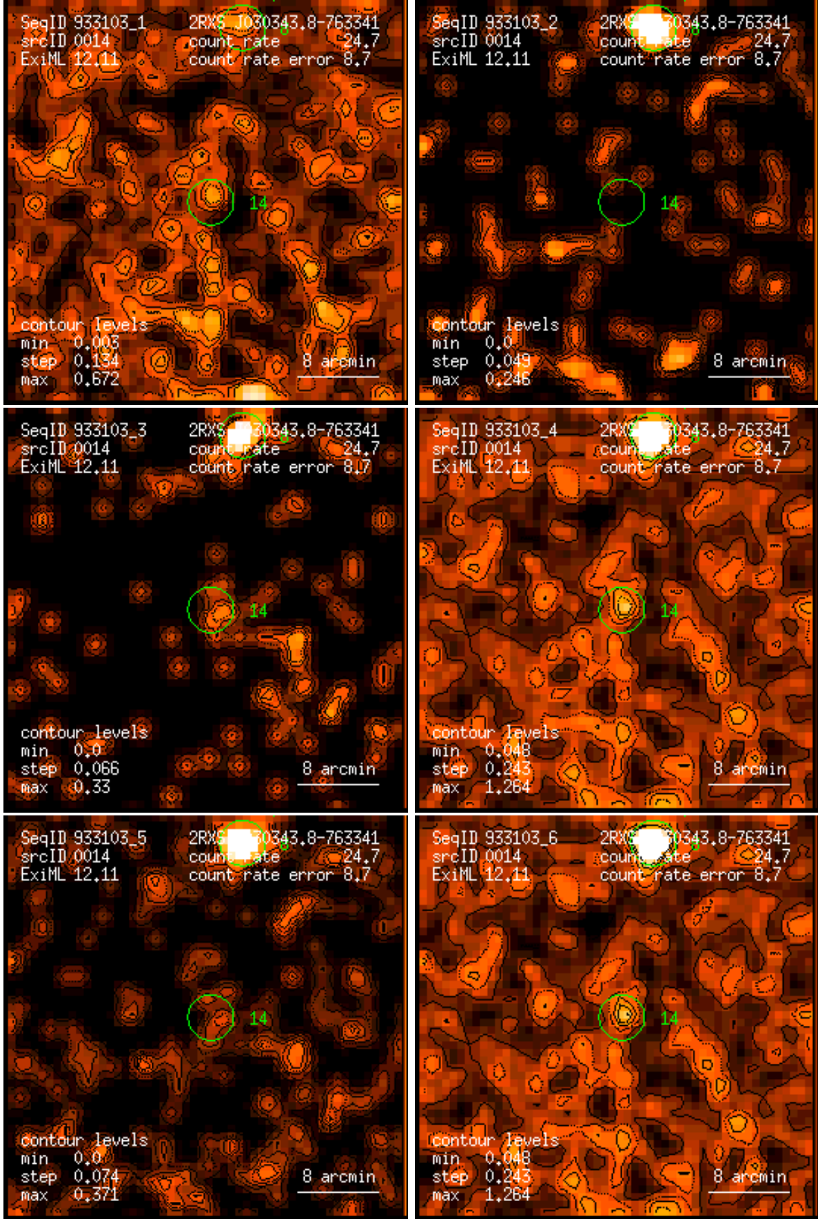
Figure 14: RASS 933103: detection 0014: band rate images, Gaussian filter: (1) PSPC channels 11 – 41, (2) 52 – 90, (3) 91 – 201, (4) 11 – 235, (5) 52 – 201, (6) 11 – 201. Broad band rates in counts/ks. Band rate contour levels in counts/ks/arcmin 2 .
