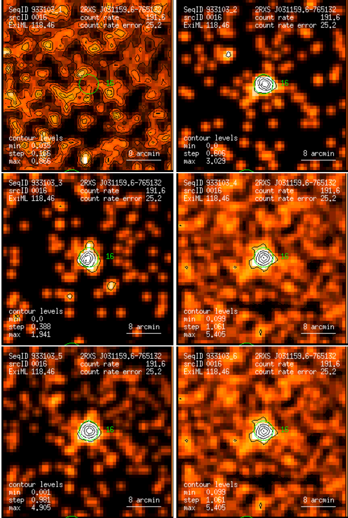
Figure 16: RASS 933103: detection 0016: band rate images, Gaussian filter: (1) PSPC channels 11 – 41, (2) 52 – 90, (3) 91 – 201, (4) 11 – 235, (5) 52 – 201, (6) 11 – 201. Broad band rates in counts/ks. Band rate contour levels in counts/ks/arcmin 2 .
