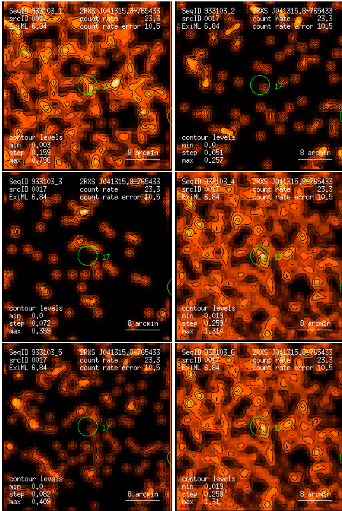
Figure 17: RASS 933103: detection 0017: band rate images, Gaussian filter: (1) PSPC channels 11 – 41, (2) 52 – 90, (3) 91 – 201, (4) 11 – 235, (5) 52 – 201, (6) 11 – 201. Broad band rates in counts/ks. Band rate contour levels in counts/ks/arcmin 2 .
