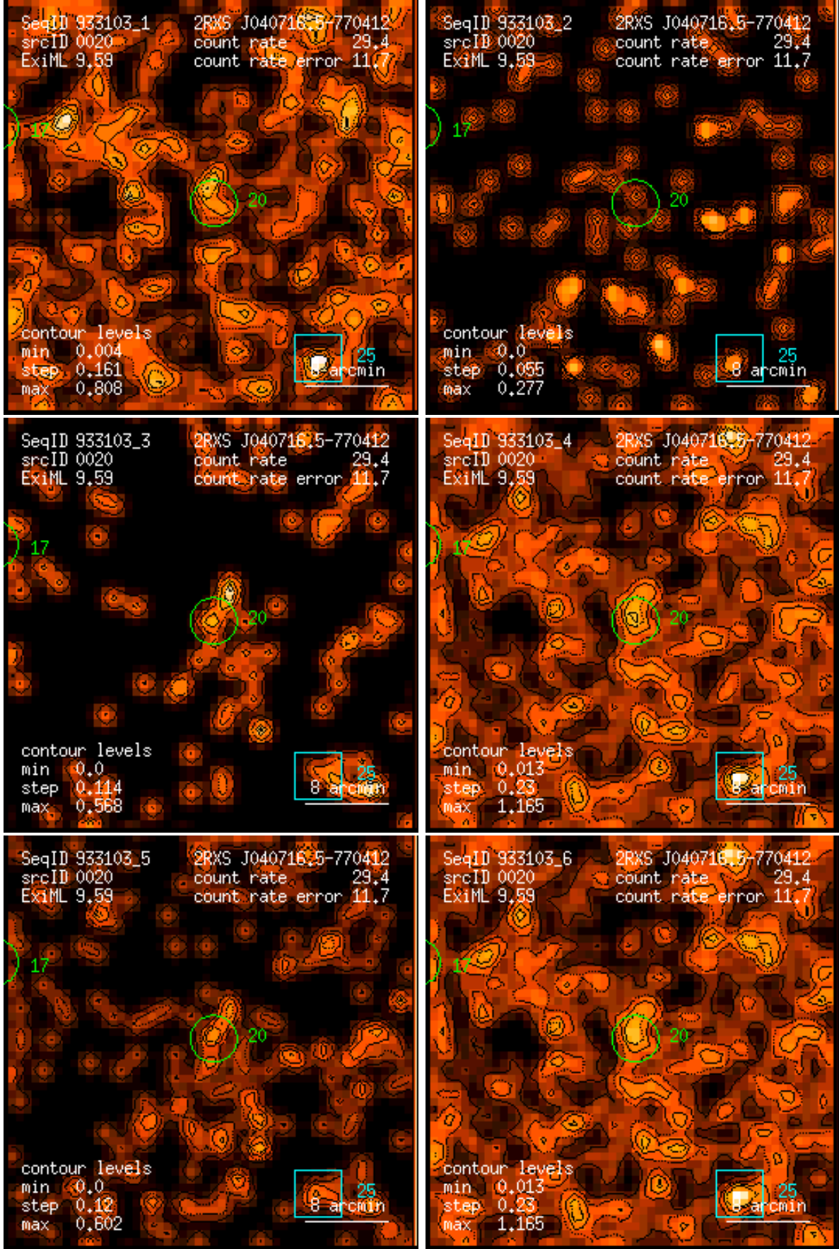
Figure 20: RASS 933103: detection 0020: band rate images, Gaussian filter: (1) PSPC channels 11 – 41, (2) 52 – 90, (3) 91 – 201, (4) 11 – 235, (5) 52 – 201, (6) 11 – 201. Broad band rates in counts/ks. Band rate contour levels in counts/ks/arcmin 2 .
