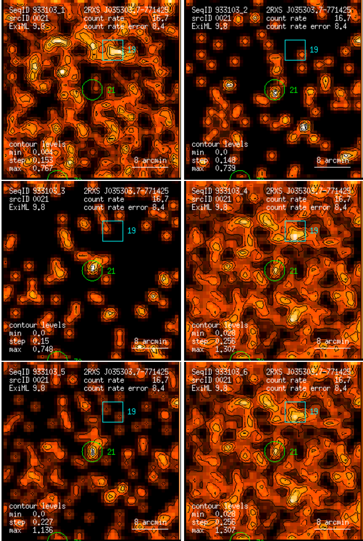
Figure 21: RASS 933103: detection 0021: band rate images, Gaussian filter: (1) PSPC channels 11 – 41, (2) 52 – 90, (3) 91 – 201, (4) 11 – 235, (5) 52 – 201, (6) 11 – 201. Broad band rates in counts/ks. Band rate contour levels in counts/ks/arcmin 2 .
