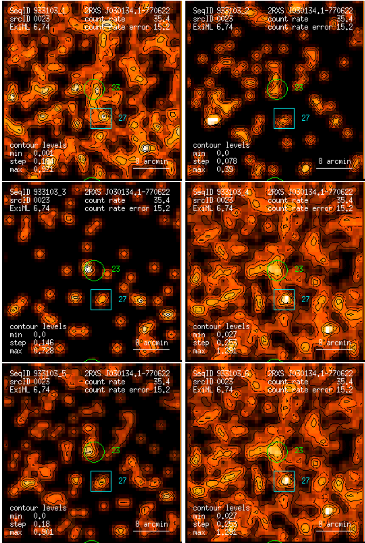
Figure 23: RASS 933103: detection 0023: band rate images, Gaussian filter: (1) PSPC channels 11 – 41, (2) 52 – 90, (3) 91 – 201, (4) 11 – 235, (5) 52 – 201, (6) 11 – 201. Broad band rates in counts/ks. Band rate contour levels in counts/ks/arcmin 2 .
