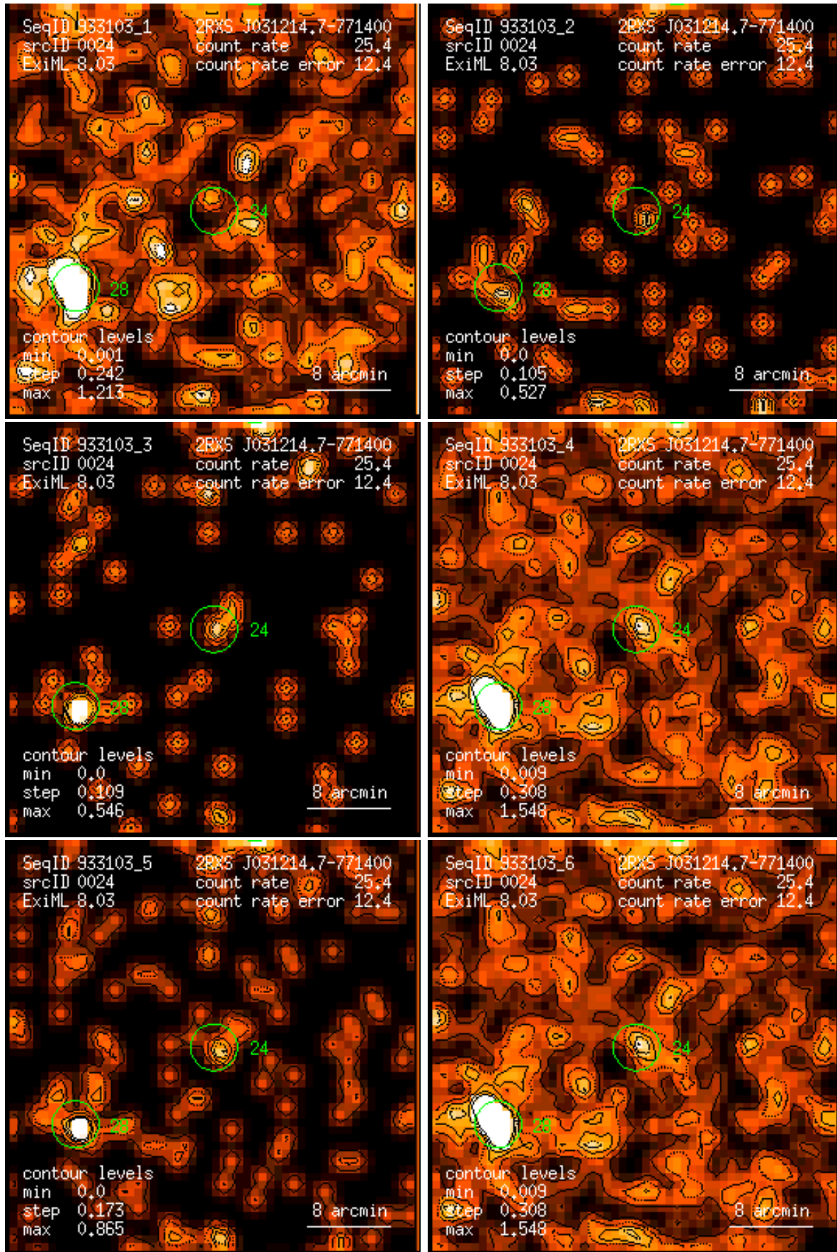
Figure 24: RASS 933103: detection 0024: band rate images, Gaussian filter: (1) PSPC channels 11 – 41, (2) 52 – 90, (3) 91 – 201, (4) 11 – 235, (5) 52 – 201, (6) 11 – 201. Broad band rates in counts/ks. Band rate contour levels in counts/ks/arcmin 2 .
