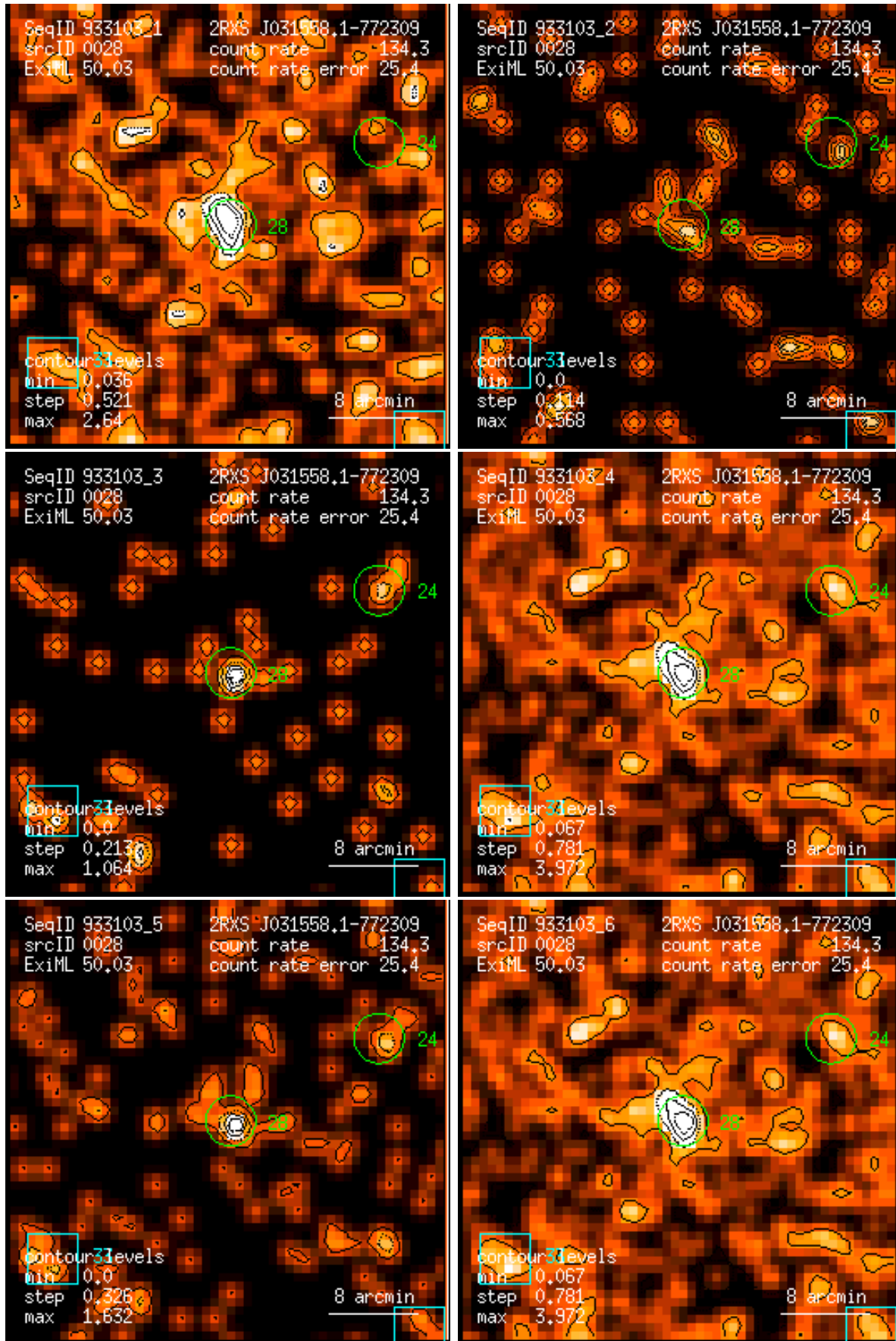
Figure 28: RASS 933103: detection 0028: band rate images, Gaussian filter: (1) PSPC channels 11 – 41, (2) 52 – 90, (3) 91 – 201, (4) 11 – 235, (5) 52 – 201, (6) 11 – 201. Broad band rates in counts/ks. Band rate contour levels in counts/ks/arcmin 2 .
