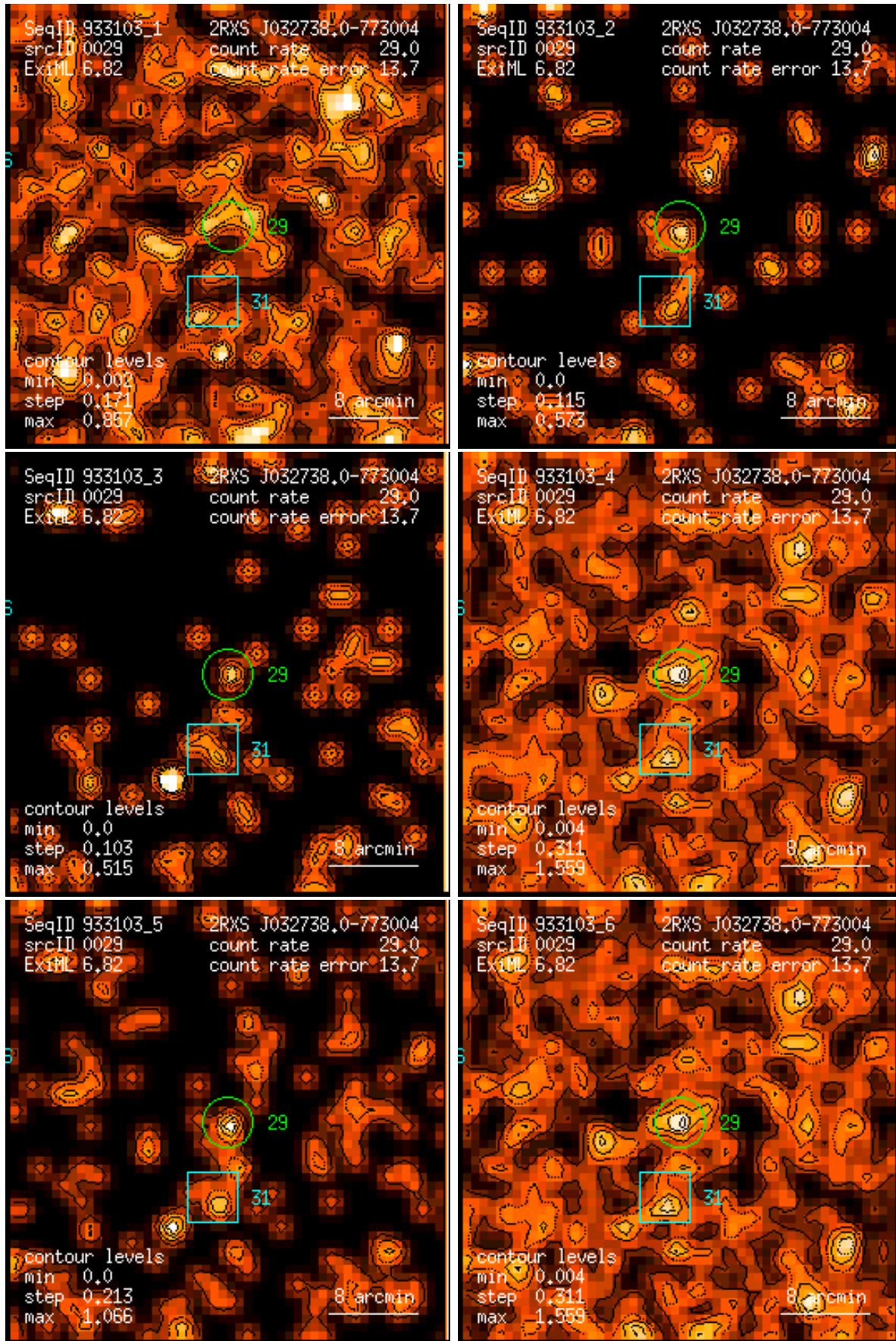
Figure 29: RASS 933103: detection 0029: band rate images, Gaussian filter: (1) PSPC channels 11 – 41, (2) 52 – 90, (3) 91 – 201, (4) 11 – 235, (5) 52 – 201, (6) 11 – 201. Broad band rates in counts/ks. Band rate contour levels in counts/ks/arcmin 2 .
