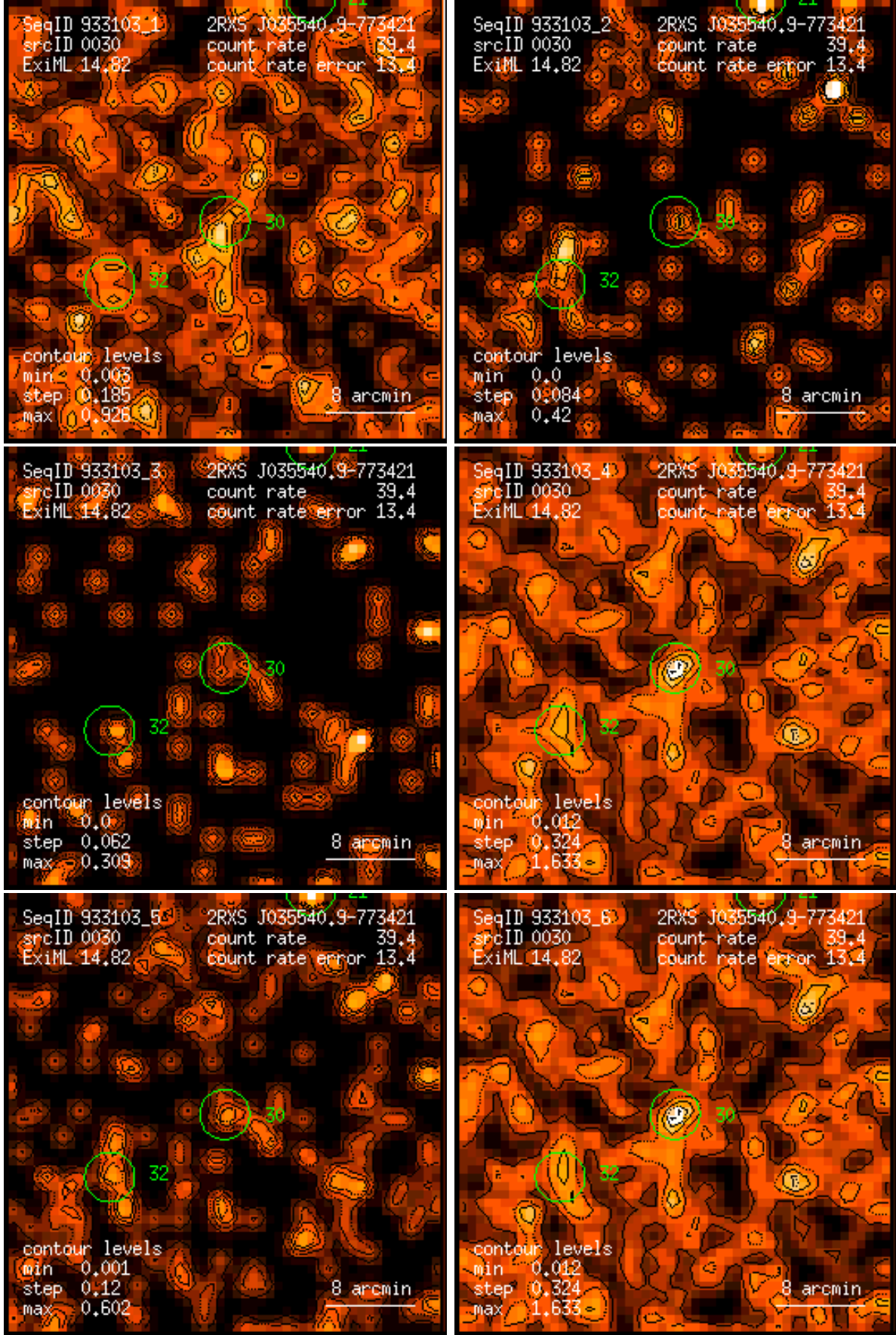
Figure 30: RASS 933103: detection 0030: band rate images, Gaussian filter: (1) PSPC channels 11 – 41, (2) 52 – 90, (3) 91 – 201, (4) 11 – 235, (5) 52 – 201, (6) 11 – 201. Broad band rates in counts/ks. Band rate contour levels in counts/ks/arcmin 2 .
