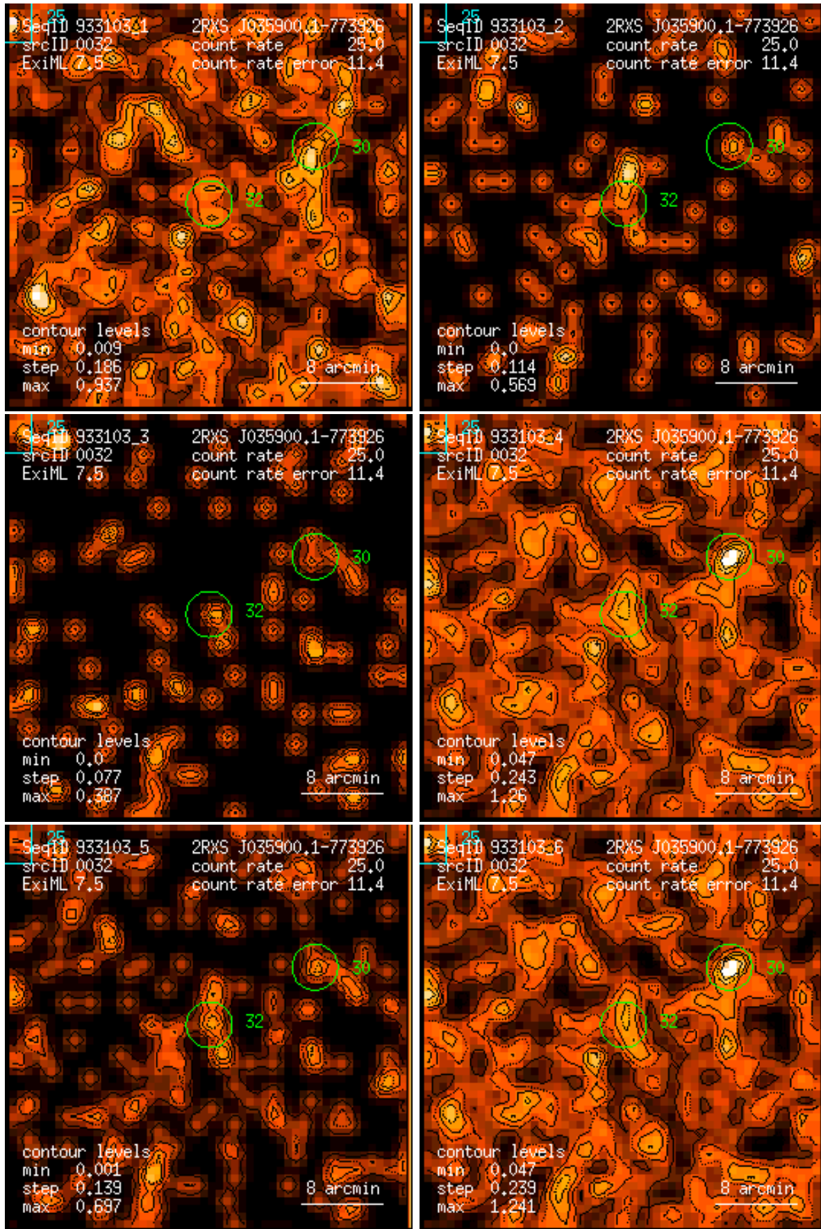
Figure 32: RASS 933103: detection 0032: band rate images, Gaussian filter: (1) PSPC channels 11 – 41, (2) 52 – 90, (3) 91 – 201, (4) 11 – 235, (5) 52 – 201, (6) 11 – 201. Broad band rates in counts/ks. Band rate contour levels in counts/ks/arcmin 2 .
