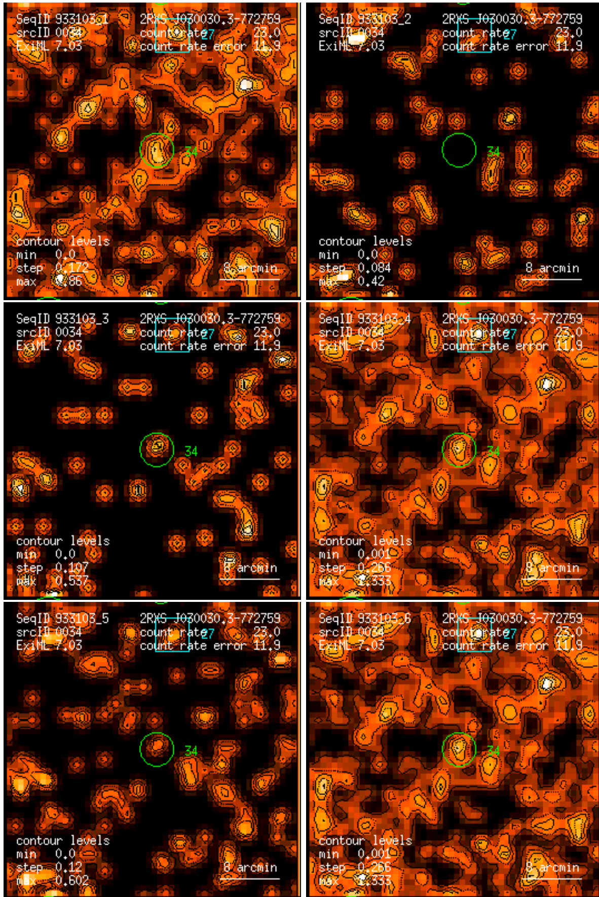
Figure 34: RASS 933103: detection 0034: band rate images, Gaussian filter: (1) PSPC channels 11 – 41, (2) 52 – 90, (3) 91 – 201, (4) 11 – 235, (5) 52 – 201, (6) 11 – 201. Broad band rates in counts/ks. Band rate contour levels in counts/ks/arcmin 2 .
