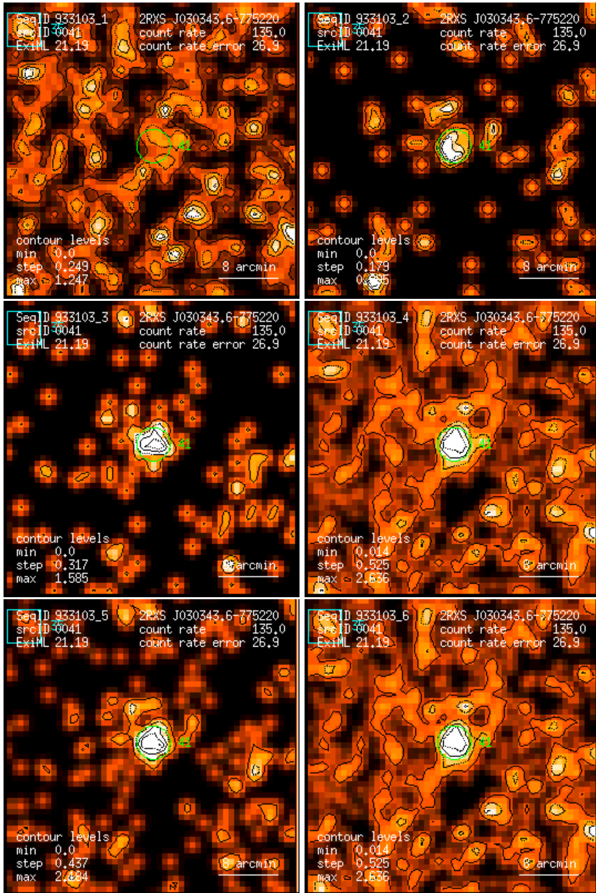
Figure 41: RASS 933103: detection 0041: band rate images, Gaussian filter: (1) PSPC channels 11 – 41, (2) 52 – 90, (3) 91 – 201, (4) 11 – 235, (5) 52 – 201, (6) 11 – 201. Broad band rates in counts/ks. Band rate contour levels in counts/ks/arcmin 2 .
