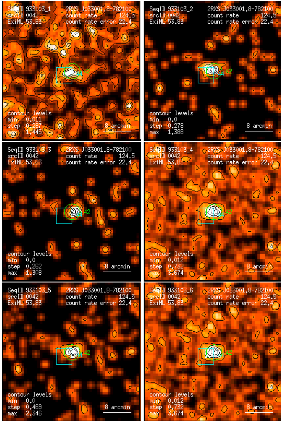
Figure 42: RASS 933103: detection 0042: band rate images, Gaussian filter: (1) PSPC channels 11 – 41, (2) 52 – 90, (3) 91 – 201, (4) 11 – 235, (5) 52 – 201, (6) 11 – 201. Broad band rates in counts/ks. Band rate contour levels in counts/ks/arcmin 2 .
