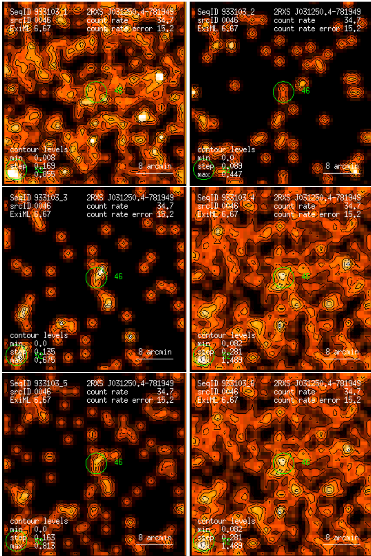
Figure 46: RASS 933103: detection 0046: band rate images, Gaussian filter: (1) PSPC channels 11 – 41, (2) 52 – 90, (3) 91 – 201, (4) 11 – 235, (5) 52 – 201, (6) 11 – 201. Broad band rates in counts/ks. Band rate contour levels in counts/ks/arcmin 2 .
