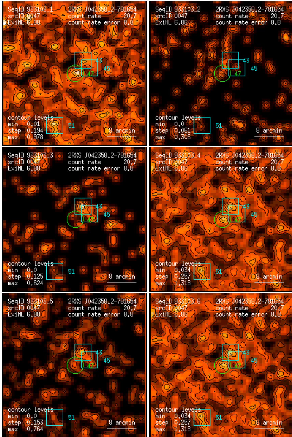
Figure 47: RASS 933103: detection 0047: band rate images, Gaussian filter: (1) PSPC channels 11 – 41, (2) 52 – 90, (3) 91 – 201, (4) 11 – 235, (5) 52 – 201, (6) 11 – 201. Broad band rates in counts/ks. Band rate contour levels in counts/ks/arcmin 2 .
