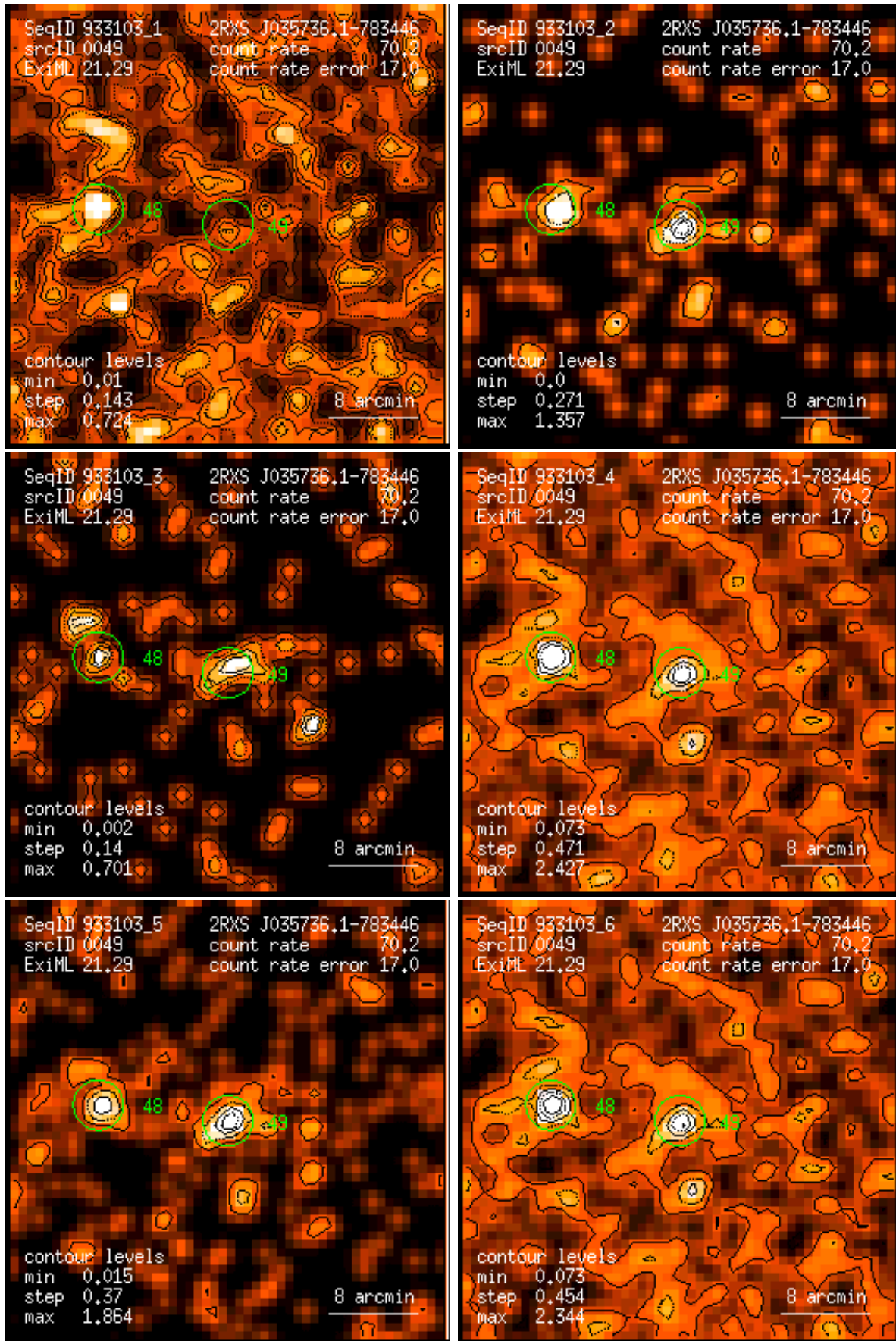
Figure 49: RASS 933103: detection 0049: band rate images, Gaussian filter: (1) PSPC channels 11 – 41, (2) 52 – 90, (3) 91 – 201, (4) 11 – 235, (5) 52 – 201, (6) 11 – 201. Broad band rates in counts/ks. Band rate contour levels in counts/ks/arcmin 2 .
