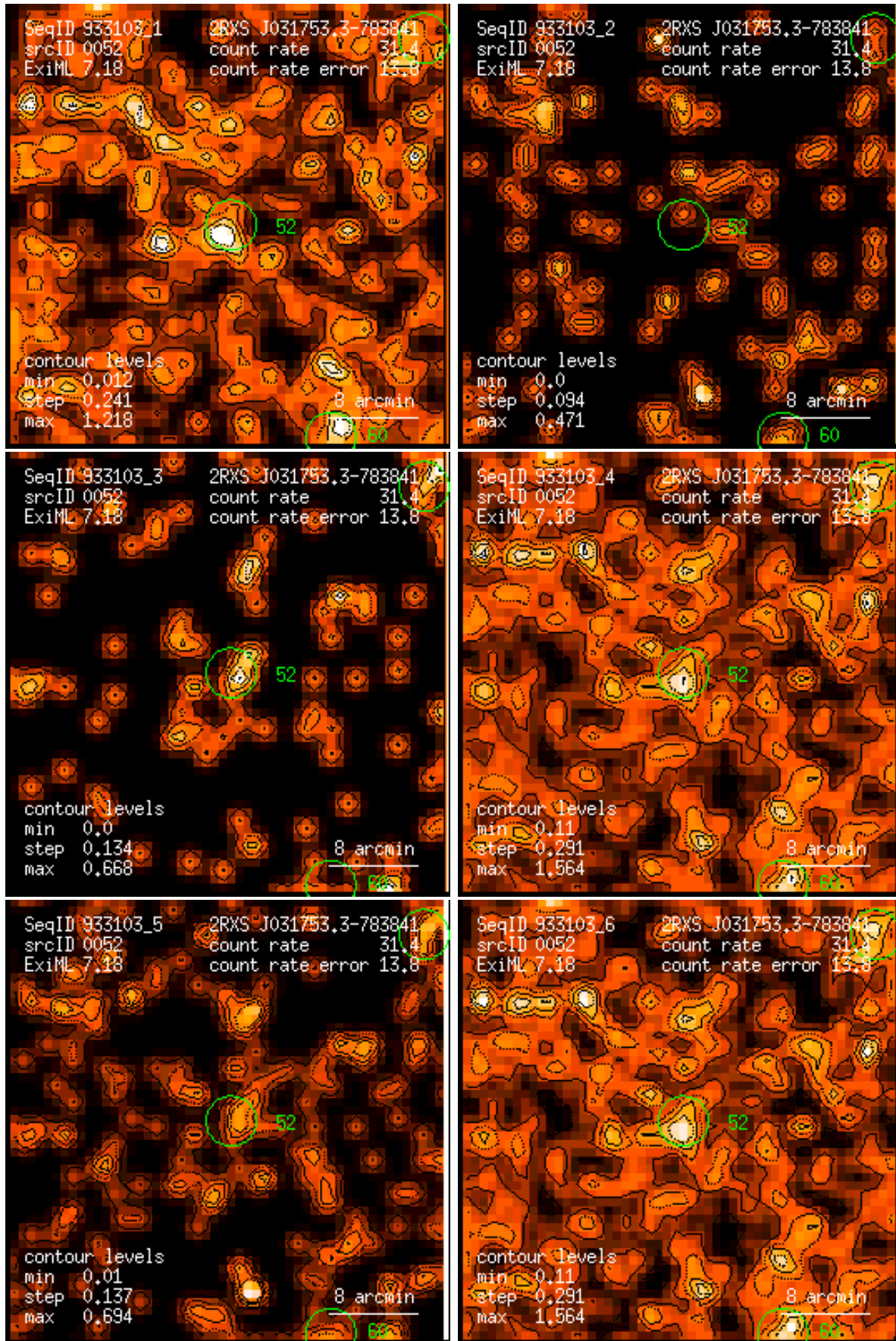
Figure 52: RASS 933103: detection 0052: band rate images, Gaussian filter: (1) PSPC channels 11 – 41, (2) 52 – 90, (3) 91 – 201, (4) 11 – 235, (5) 52 – 201, (6) 11 – 201. Broad band rates in counts/ks. Band rate contour levels in counts/ks/arcmin 2 .
