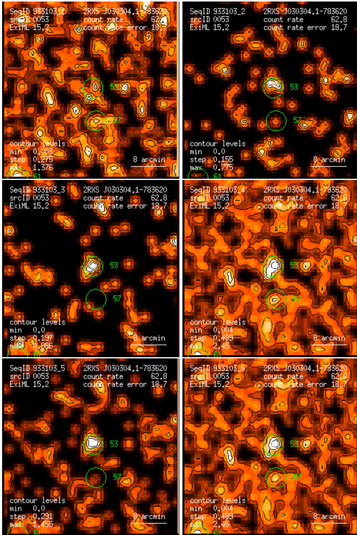
Figure 53: RASS 933103: detection 0053: band rate images, Gaussian filter: (1) PSPC channels 11 – 41, (2) 52 – 90, (3) 91 – 201, (4) 11 – 235, (5) 52 – 201, (6) 11 – 201. Broad band rates in counts/ks. Band rate contour levels in counts/ks/arcmin 2 .
