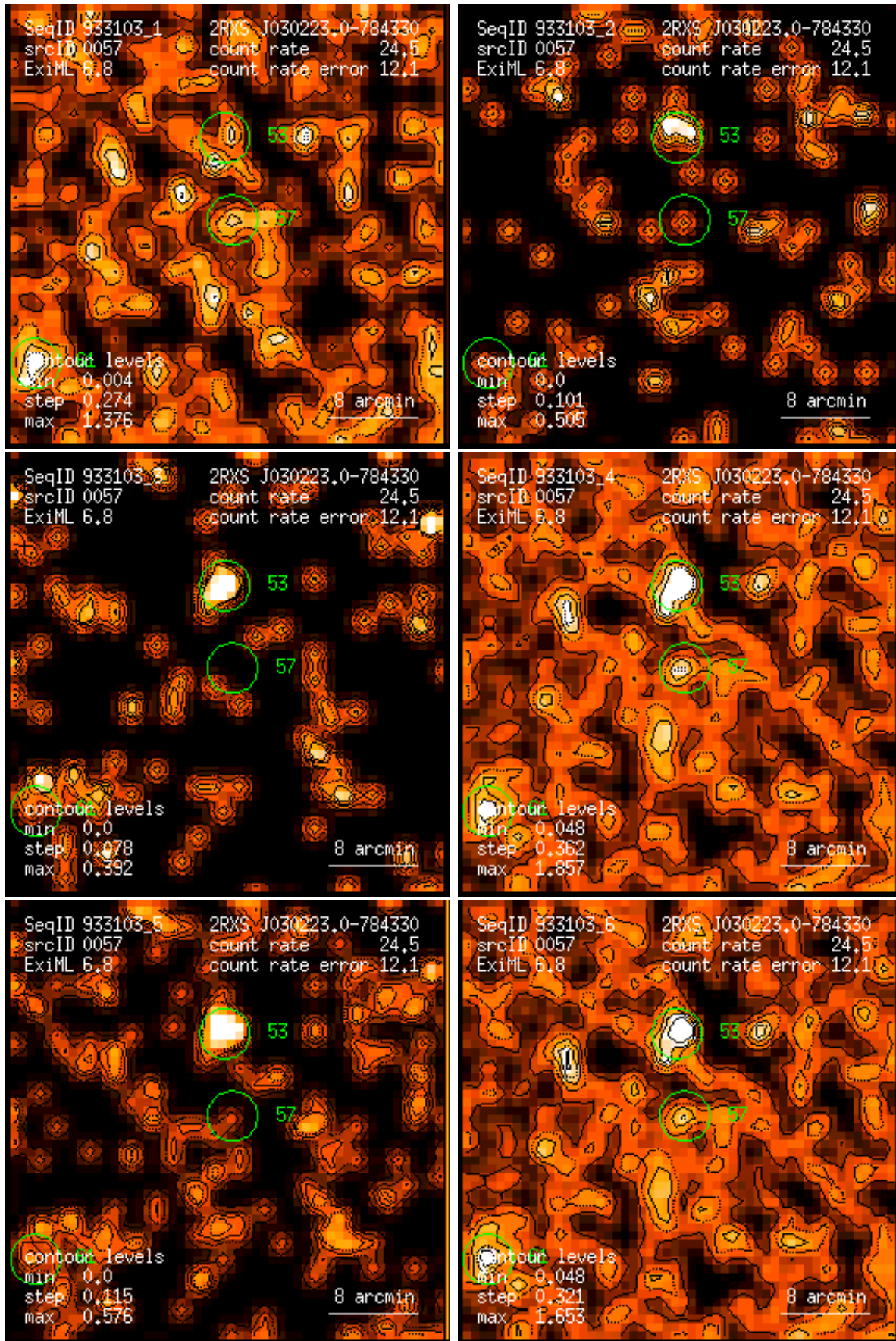
Figure 57: RASS 933103: detection 0057: band rate images, Gaussian filter: (1) PSPC channels 11 – 41, (2) 52 – 90, (3) 91 – 201, (4) 11 – 235, (5) 52 – 201, (6) 11 – 201. Broad band rates in counts/ks. Band rate contour levels in counts/ks/arcmin 2 .
