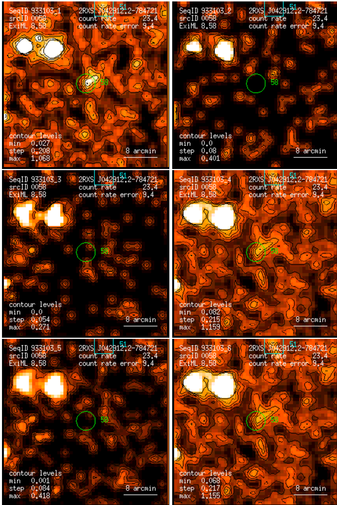
Figure 58: RASS 933103: detection 0058: band rate images, Gaussian filter: (1) PSPC channels 11 – 41, (2) 52 – 90, (3) 91 – 201, (4) 11 – 235, (5) 52 – 201, (6) 11 – 201. Broad band rates in counts/ks. Band rate contour levels in counts/ks/arcmin 2 .
