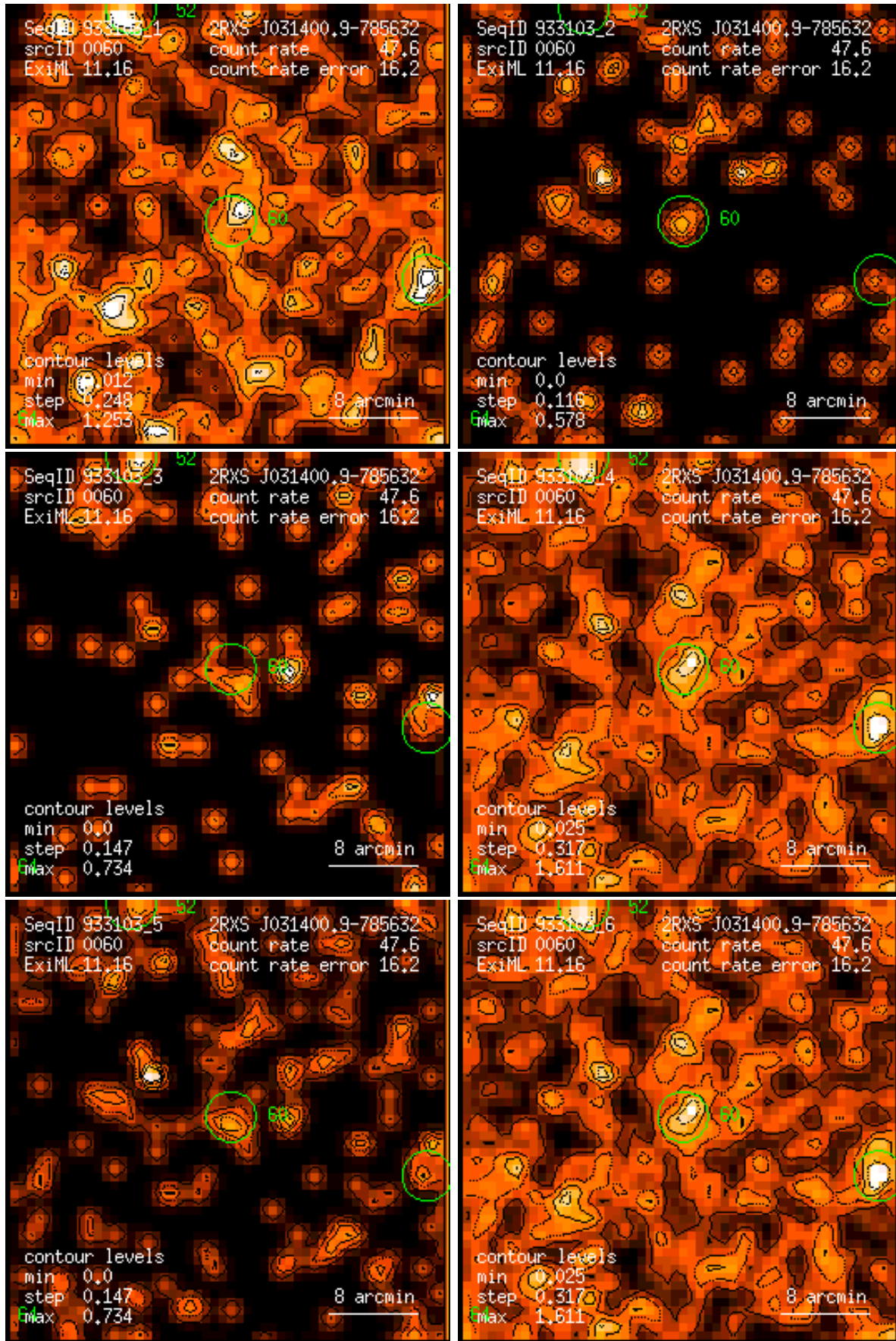
Figure 60: RASS 933103: detection 0060: band rate images, Gaussian filter: (1) PSPC channels 11 – 41, (2) 52 – 90, (3) 91 – 201, (4) 11 – 235, (5) 52 – 201, (6) 11 – 201. Broad band rates in counts/ks. Band rate contour levels in counts/ks/arcmin 2 .
