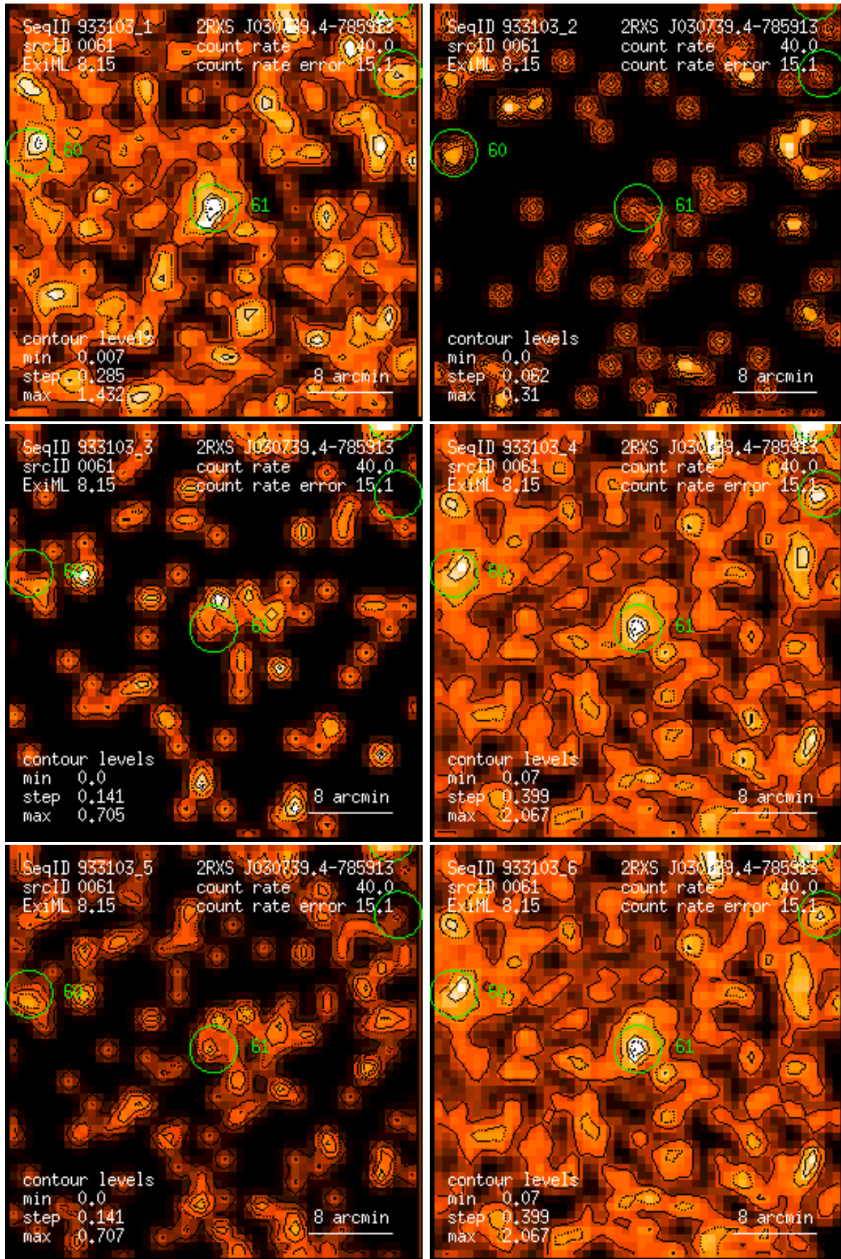
Figure 61: RASS 933103: detection 0061: band rate images, Gaussian filter: (1) PSPC channels 11 – 41, (2) 52 – 90, (3) 91 – 201, (4) 11 – 235, (5) 52 – 201, (6) 11 – 201. Broad band rates in counts/ks. Band rate contour levels in counts/ks/arcmin 2 .
