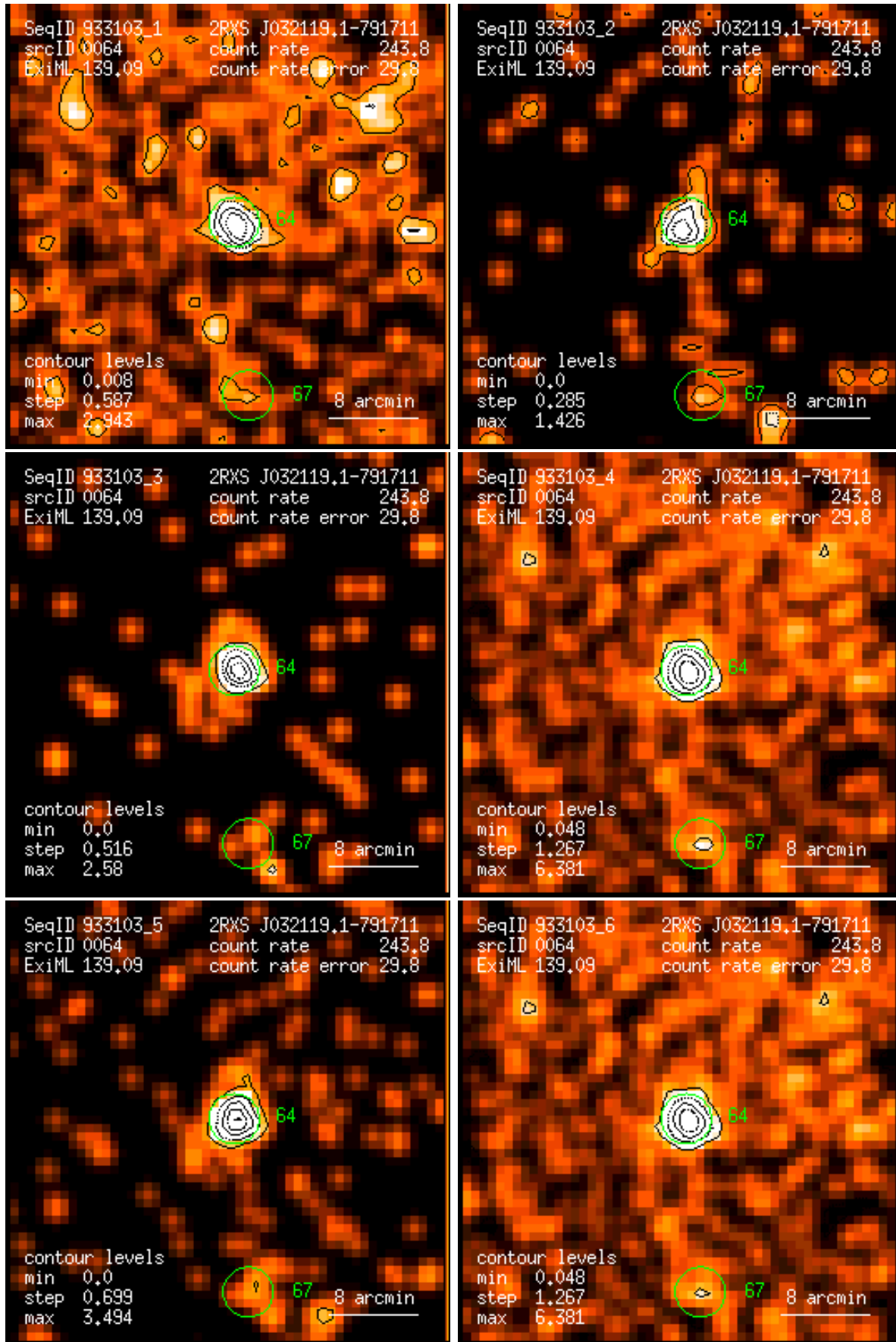
Figure 64: RASS 933103: detection 0064: band rate images, Gaussian filter: (1) PSPC channels 11 – 41, (2) 52 – 90, (3) 91 – 201, (4) 11 – 235, (5) 52 – 201, (6) 11 – 201. Broad band rates in counts/ks. Band rate contour levels in counts/ks/arcmin 2 .
