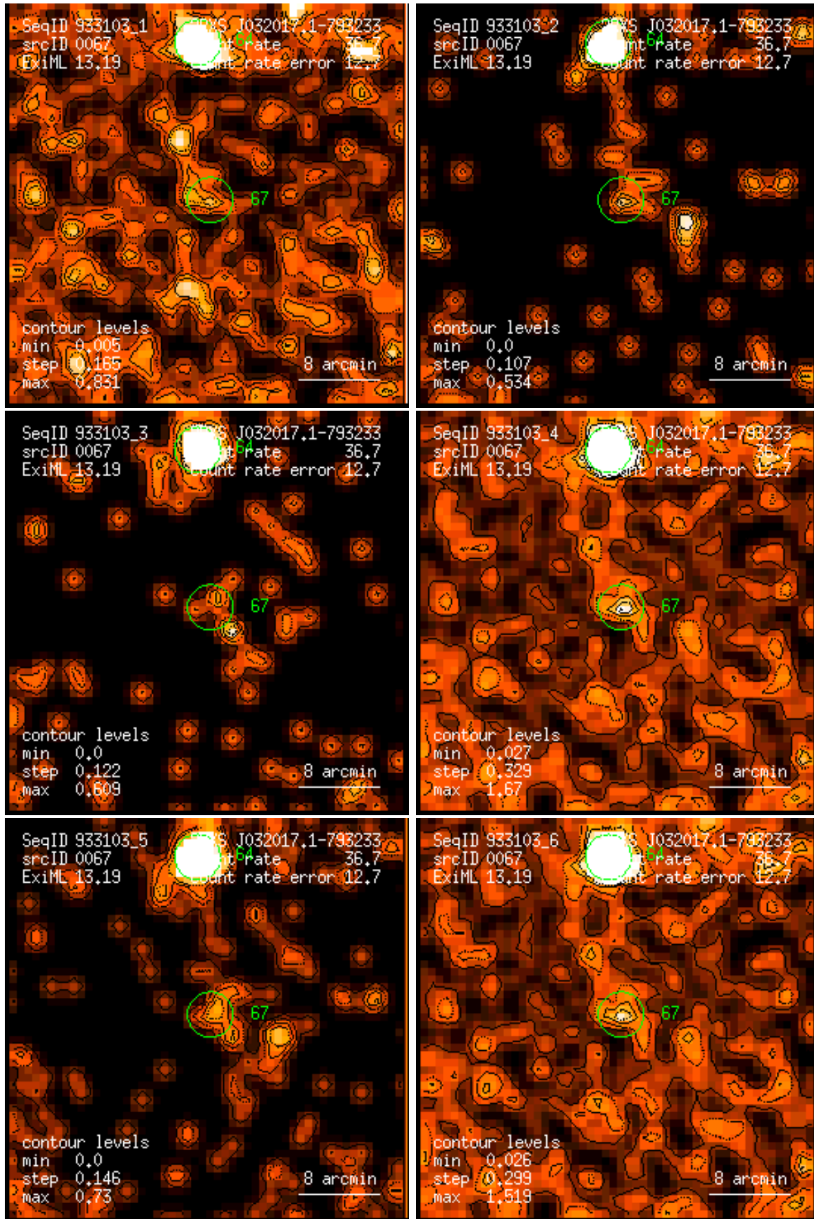
Figure 67: RASS 933103: detection 0067: band rate images, Gaussian filter: (1) PSPC channels 11 – 41, (2) 52 – 90, (3) 91 – 201, (4) 11 – 235, (5) 52 – 201, (6) 11 – 201. Broad band rates in counts/ks. Band rate contour levels in counts/ks/arcmin 2 .
