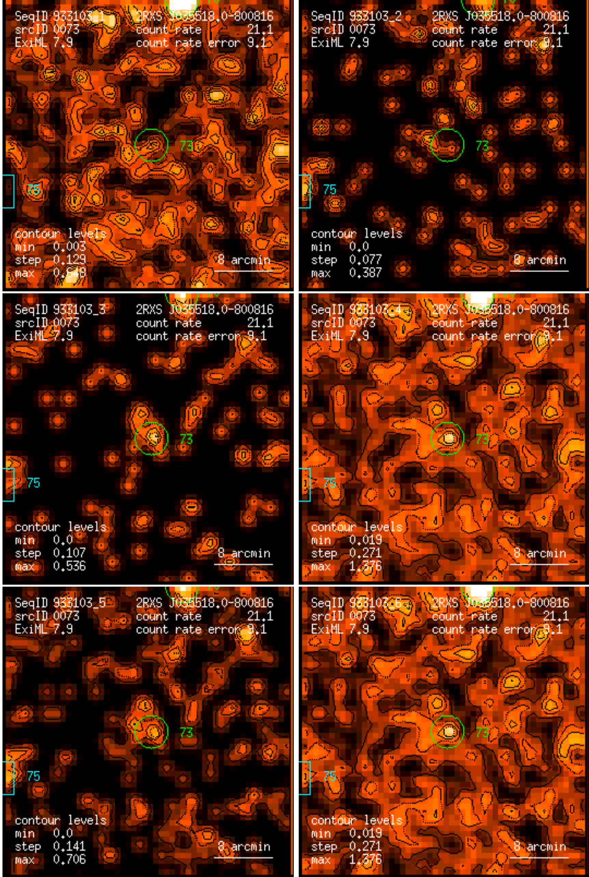
Figure 73: RASS 933103: detection 0073: band rate images, Gaussian filter: (1) PSPC channels 11 – 41, (2) 52 – 90, (3) 91 – 201, (4) 11 – 235, (5) 52 – 201, (6) 11 – 201. Broad band rates in counts/ks. Band rate contour levels in counts/ks/arcmin 2 .
