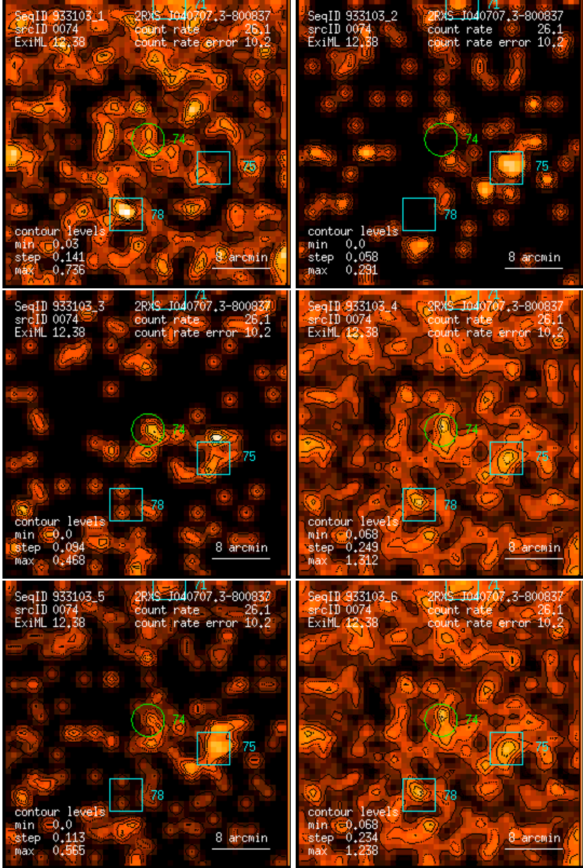
Figure 74: RASS 933103: detection 0074: band rate images, Gaussian filter: (1) PSPC channels 11 – 41, (2) 52 – 90, (3) 91 – 201, (4) 11 – 235, (5) 52 – 201, (6) 11 – 201. Broad band rates in counts/ks. Band rate contour levels in counts/ks/arcmin 2 .
